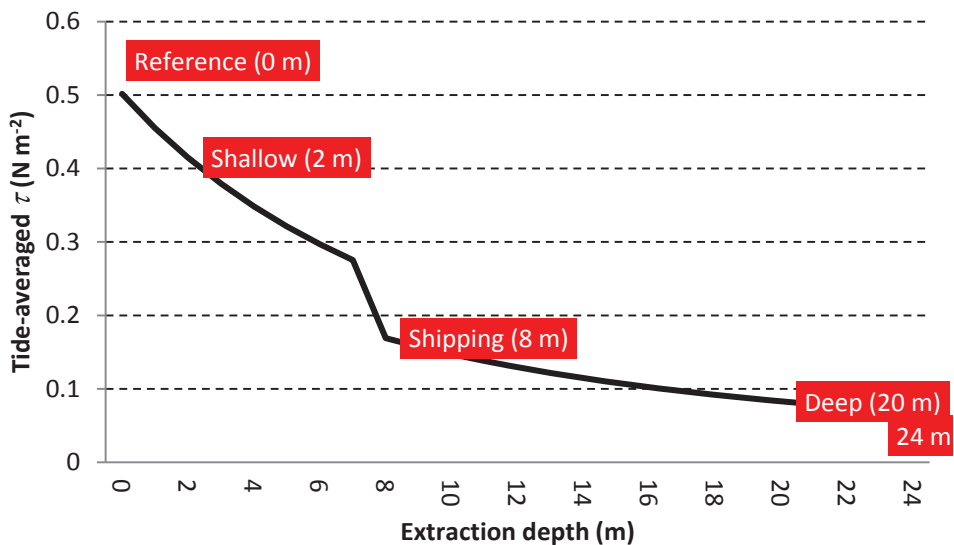
Fig. 5.4 Tide-averaged bed shear stress ( \tau_{b \text{ tide-averaged}} ) as a function of sand extraction depth at 20 m pre-extraction water depth and using a Chézy roughness value of 65 \text{m}^{1/2}/\text{s} for sand extraction depth interval 0–8 m, 80 \text{m}^{1/2}/\text{s} for 8–20 m and 110 \text{m}^{1/2}/\text{s} for the deepest extraction depth. The reference situation and case studies (shallow sand extraction, shipping lane and deep sand extraction: 20 and 24 m) are indicated with the red text labels.
