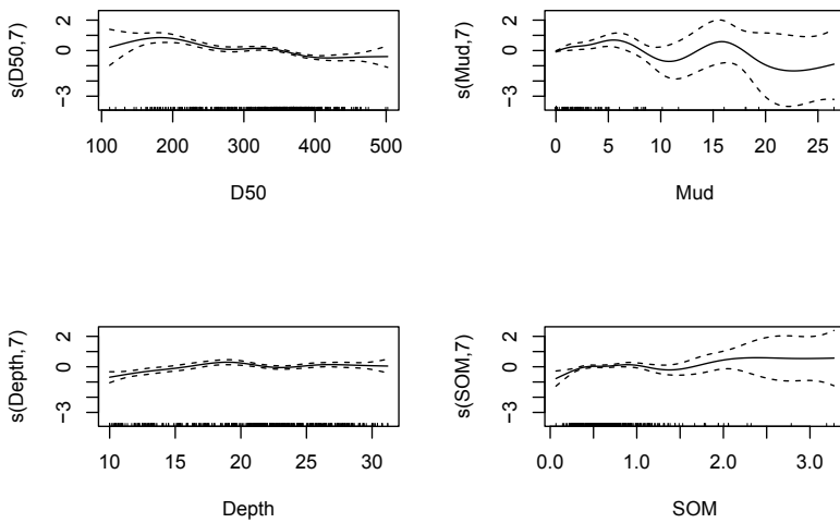
Figure 2.7 Response curves of infaunal biomass (log10 transformed) and significant continuous variables
