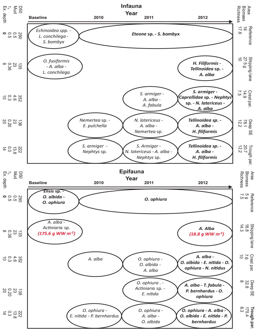
Figure 3.16 Summary of infaunal and epifaunal species composition and biomass in relation to D 50 , mud content, mean near-bed shear stress ( \tau_b ) and excavation depth.
