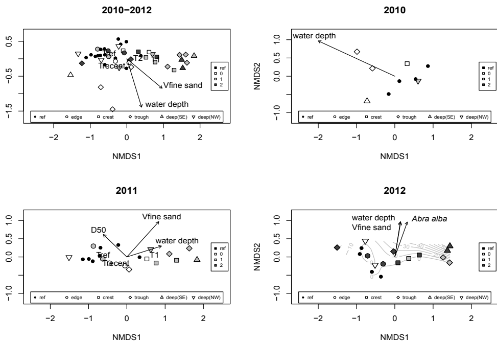
Figure 4.6 nMDS ordination with sites and significant associations with variables. Continuous variables are depicted with arrows and categorical variable time after the cessation, only with text ( t_{ref} : reference in black, t_{recent} in white, t_1 in light grey and t_2 in dark grey). Sub locations are denoted with symbols, reference as black bullets, slope of the reference area as open large circles, crests of sandbars as squares, trough of sandbars as diamonds, deep (SE) as point-up triangles and deep (NW) as point-down triangles. In 2012, the significant association of the ordination and infaunal white furrow shell biomass is denoted with an arrow and surface plot to show the non-linearity. Stress of all ordinations was below 0.07.
