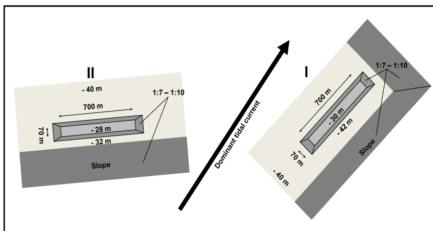
Figure 4.2 Schematic representation of the ecosystem-based landscaped sandbars, left: sandbar II, oblique to the tidal current and right: sandbar I, parallel to the tidal current.
