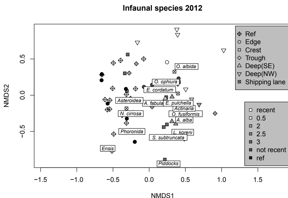
Figure 3.11 2-D ordination plot of 2012 (first 2 axis) with most abundant or characteristic species.
