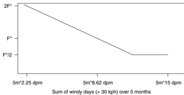
Figure 3. Fishing pressure of the EHCR as a function of the number of windy days during the 5 months (May to September) with highest proportion of juveniles younger than 3 months. The number of easterly windy days per month (dpm) is uniformly distributed on the interval [2.25,15]. The average number of windy days per month is 8.62, the average number of the easterly windy days for the entire period is 5 m*8.62 dpm.
