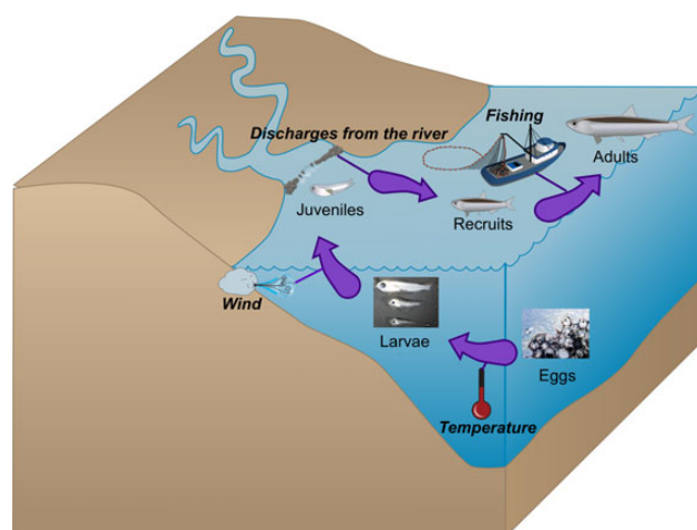
Figure 1. Diagram of anchovy life cycle in the Gulf of Cádiz including environmental factors affecting different life stages. Courtesy of the Integration and Application Network, University of Maryland Center for Environmental Science (ian.umces.edu/symbols/). This figure is available in black and white in print and in colour at ICES Journal of Marine Science online.
