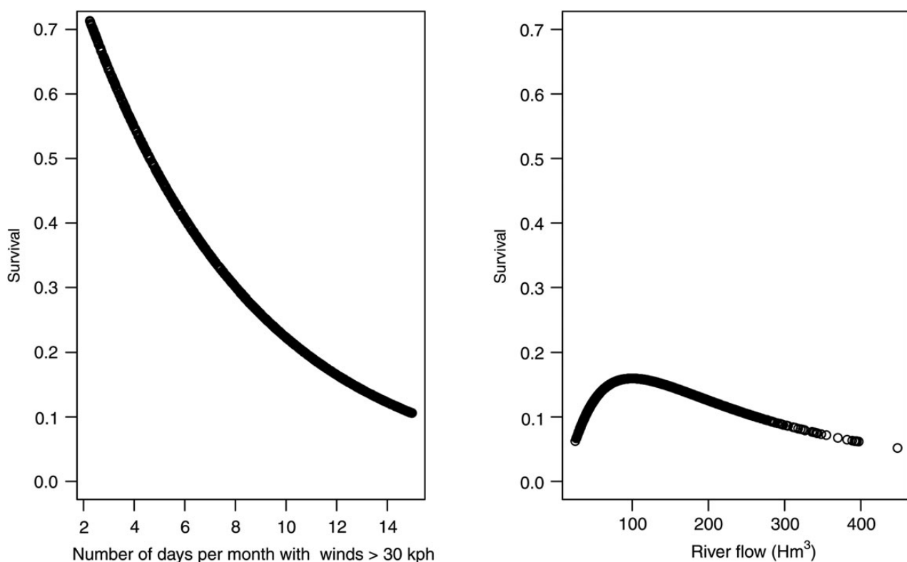
Figure 2. Left: Effect of strong easterly winds on survival after one month for 1000 values of simulated wind values. Right: Effect of discharges on survival after 1 month for 1000 values of simulated discharges.
