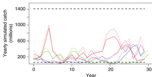
Figure 5. Four samples of simulated catches under two regimes in the base model, with the fixed HCR (solid lines) and with the EHCR (dotted lines). The black dashed lines represent minimum and maximum of annual catches in millions of individual fish registered by ICES for the years 1988 to 2013.
