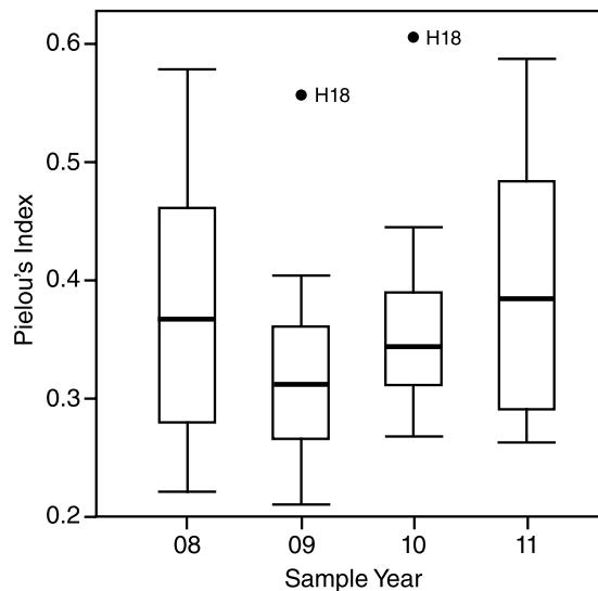
Figure 7. Boxplot of Pielou's Evenness Index for the four sampling intervals. Band inside box = mean. Whiskers = \pm 1.5 \times \text{Interquartile range (IQR)} and points represent sample sites that fall outside whiskers.
