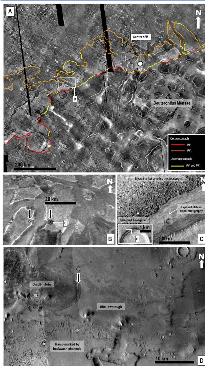
Figure 2. (A) View of highland surfaces along the highland-lowland boundary in northwestern Arabia Terra, which are embayed by the upper reaches of members IHL_1 and IHL_2 . The red ( IHL_1 ) and orange ( IHL_2 ) lines show contact sections mapped as certain. The yellow lines are zones where the contacts are obscured due to localized resurfacing or mantling. Out of the total 4124 km length of these mapped contacts, 76% is certain and 23% is uncertain. Part of THEMIS night-time infrared image mosaic (100 m/pixel) centered at 43°26'N, 12°29'E. Credit: Christensen et al. 32 . (B) Perspective close-up view on a system of mesas, which are partly covered by the upper reaches of member IHL_1 . These deposits consist of thermally bright materials that pass upland-wards into thermally dark surfaces. The black arrows show locations where the thermally dark materials are exhumed from beneath the thermally bright materials by impact craters. Center location indicated by dot in panel A. Part of THEMIS night-time infrared mosaic (100 m/pixel) centered at 45°45'N, 16°41'E. Credit: Christensen et al. 32 . (C) Visible light close-up view on one of the craters identified in panel (B). The impact crater's inner wall shows the boulder deposit (member IHL_1 ) overlying an exhumed non-bouldery upper stratigraphy. The boulder deposit is also locally covered by a non-bouldery ejecta blanket. The inset shows the view's location along the crater's northern margin. Part of HiRISE image ESP_017355_2260 centered at 45.82°N 16.47°E (50 cm/pixel). Credit: NASA/JPL/University of Arizona. (D) Close-up view of northeast Deuteronilus Mensae showing a low-angle ramp marked by backwash channels (part of member IHL_1 ), which is cut by a shallow trough. A lobe of member IHL_2 can be observed to run up the trough's surface. The black arrow identifies a marginal compressional fold. Location is shown in panel (A). Part of a CTX mosaic centered at 44°49'N, 11°10'E. Credit: NASA/JPL. The license terms can be found on the following link: pds-imaging.jpl.nasa.gov/portal/mro_mission.html . We produced the mosaics and maps in this figure using Esri's ArcGIS® 10.3 software ( http://www.esri.com/software/arcgis ).
