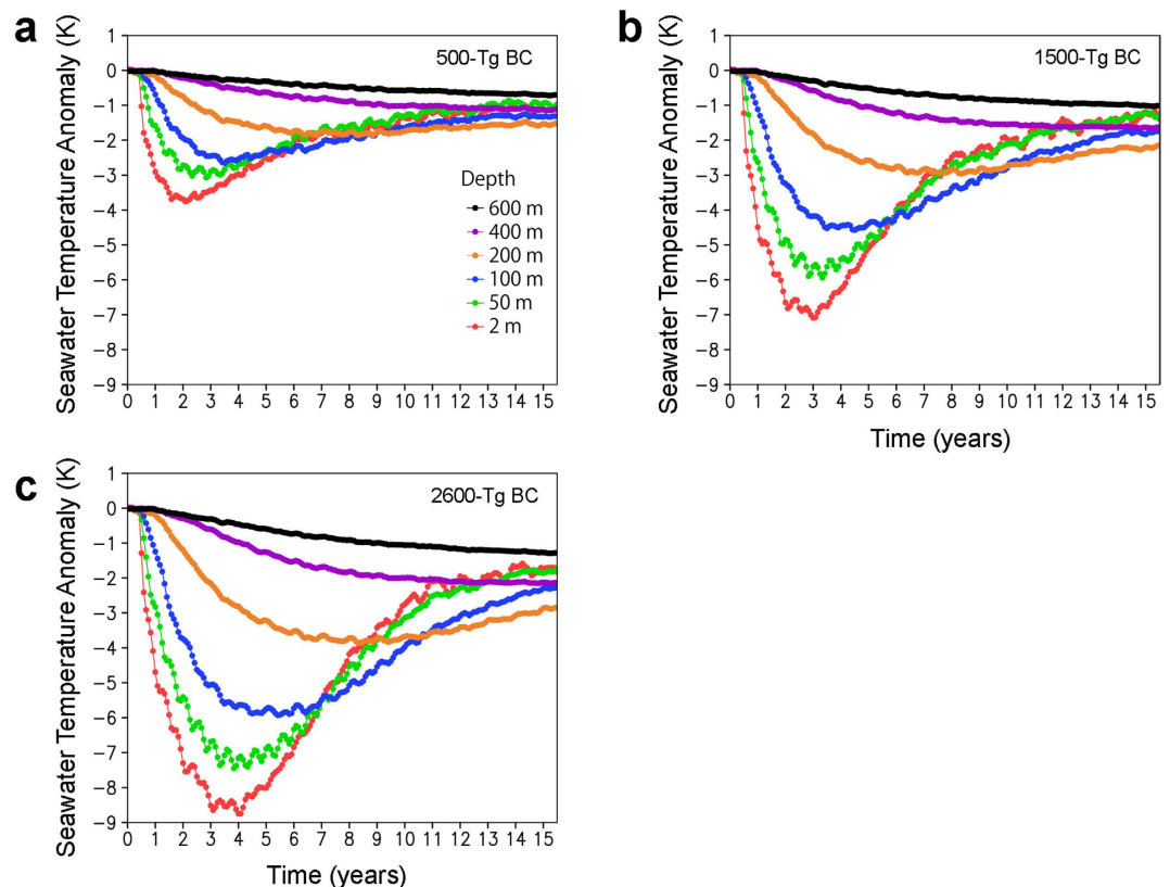
Figure 5. Seawater temperature changes caused by the black carbon (BC) injection. (a–c) Changes in the global averages of seawater temperature at 2-m, 50-m, 100-m, 200-m, 400-m, and 600-m water depths for the 500-Tg (a), 1500-Tg (b), and 2600-Tg (c) BC scenarios calculated by the climate model. Monthly anomalies from the control experiment (no ejection scenario) are shown. The 30-year global averages of seawater temperature at 2-m, 50-m, 100-m, 200-m, 400-m, and 600-m water depths in the control experiment were 293, 292, 290, 287, 283, and 280 K, respectively. The regions with seawater temperatures below zero at the 2-m water depth in the control experiment were excluded for the estimation of the anomalies and the 30-year averages to exclude the sea ice area.
