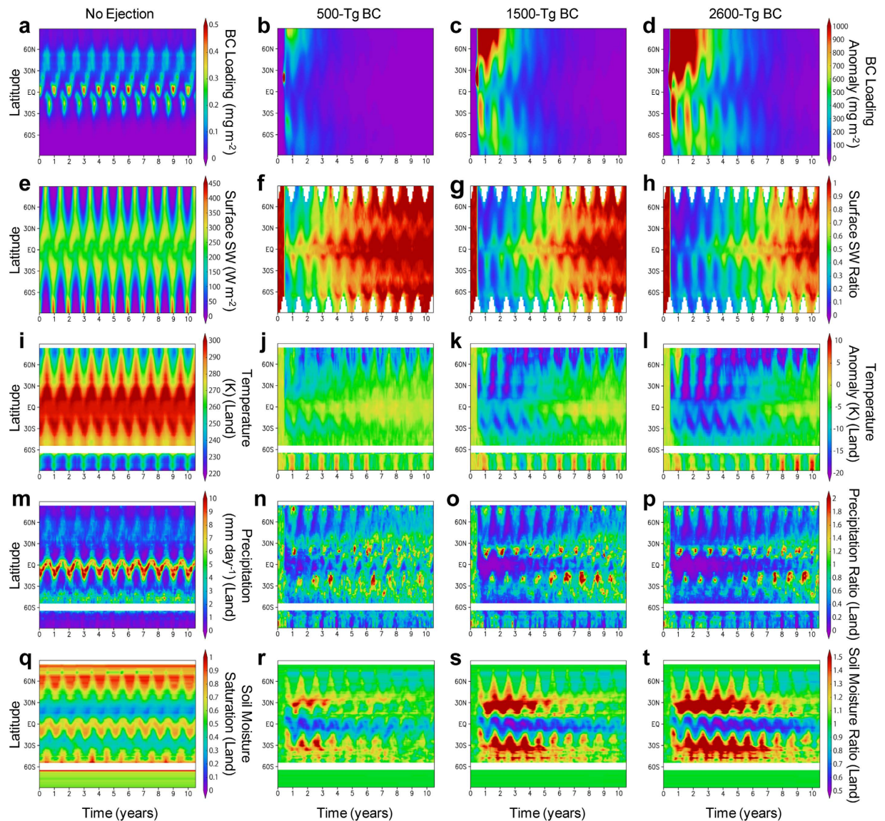
Figure 3. Meridional distributions of pre-industrial climate conditions and climate changes caused by the black carbon (BC) injection. (a–t) Time–latitude cross-sections of zonal mean changes in BC loading in the atmosphere (a–d), downward shortwave (SW) radiation at the surface (e–h), surface air temperature over land (i–l), precipitation over land (m–p), and degree of saturation of soil moisture averaged for a depth of 0–50 cm (q–t) for the no ejection (control) (a,e,i,m,q), 500-Tg (b,f,j,n,r), 1500-Tg (c,g,k,o,s), and 2600-Tg (d,h,l,p,t) BC scenarios calculated by the climate model. Monthly anomalies from the control experiment are shown for the amount of BC (b–d) and temperature (j–l). The ratios relative to the control experiment are shown for shortwave radiation (f–h), precipitation (n–p), and soil moisture (r–t). For comparison, the absolute values of the control experiment are shown (a,e,i,m,q). Regions without data correspond to those with no sunlight or the ocean. The scale for the no ejection case is different from the others. The BC emission in the no ejection case is mainly from biomass burning.
