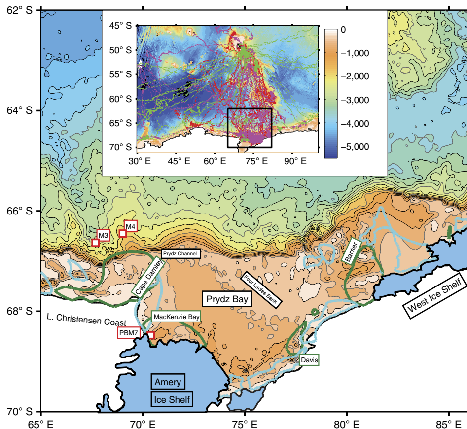
Figure 1 | Study area of Prydz Bay and surrounds. Bathymetry from ETOP01 ( http://www.ngdc.noaa.gov/mgg/global/global.html ) with 250 m contour intervals. Major geographical features shown include Prydz Bay, Prydz Channel and the Four Ladies Bank, with the Amery and West Ice Shelves. Coastal polynyas are also shown using satellite-derived sea ice production estimates (dark green contours show 5 \text{ m a}^{-1} ) from ERA-Interim data (1992–2014) 14,15 . Cape Darnley, MacKenzie Bay, Davis and Barrier Bay. Mean fast ice contours 37 are shown as thick light blue contours. Instrumented mooring locations M3, M4 (ref. 10) and PBM7 are shown with red squares. Inset: large-scale bathymetry of Southern Indian Ocean (45–72° S) across the Antarctic margin (30–100° E) with elephant seal data locations from Davis Station deployments (red and magenta points for 2011 and 2012, respectively) and an Iles Kerguelen deployment (green points from 2013). Black box indicates the location of the study area shown.
