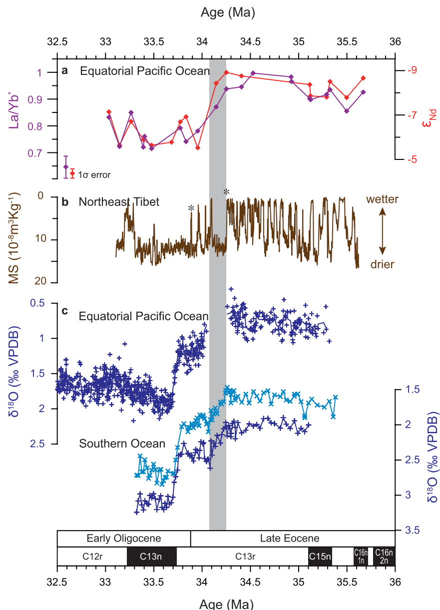
Figure 2. Inter-hemisphere changes in EOT climate. Palaeoclimate records for the Eocene-Oligocene transition from the equatorial Pacific Ocean, Northeast Tibet and the Southern Ocean. (a) \epsilon_{\text{Nd}} (red) and \text{La/Yb}^* (purple) of the inorganic silicate fraction of deep sea sediments from IODP U1334 (this study). (b) magnetic susceptibility from the Xining Basin, Tashan section (ref. 39). (c) oxygen isotope composition of benthic ( Cibicidoides spp., dark blue) and planktic ( S. angiporoides , light blue) foraminiferal calcite from ODP Sites 1218 (refs 3,22) and 689 (ref. 10). Magnetic susceptibility (MS) of the Tashan section reflects lithological change in a sequence of red mudstones (high MS) signifying arid conditions and gypsum/gypsiferous layers (low MS) that signify higher water supply. Asterisks in panel (b) show position of two tie points, in addition to magnetostratigraphic datums, used for the correlation of terrestrial to marine records (see methods).
