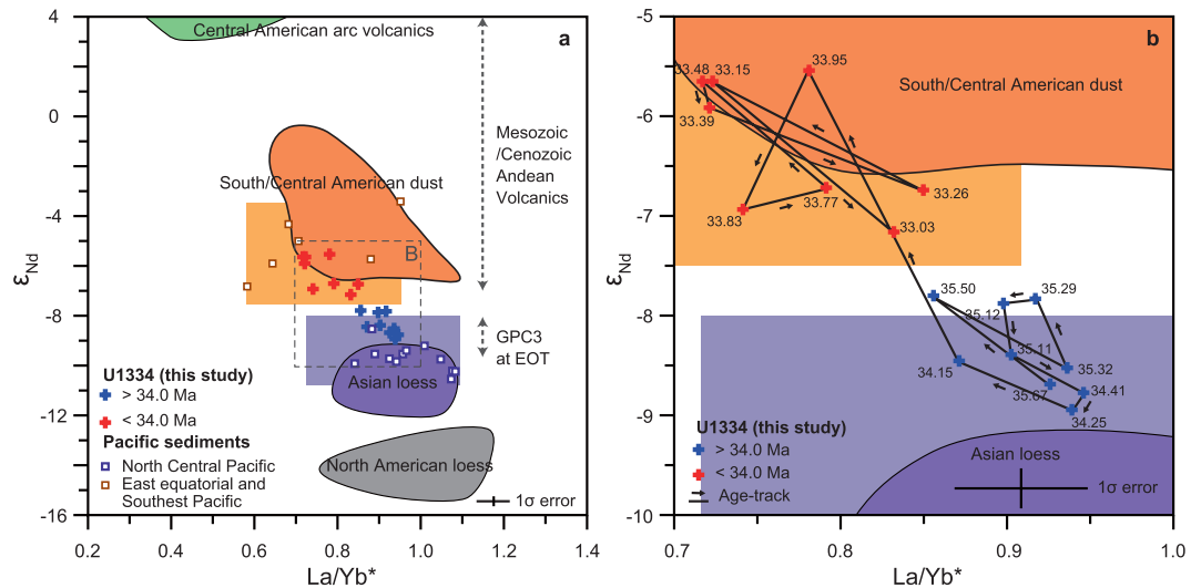
Figure 3. \epsilon_{Nd} vs. La/Yb^* . (a) \epsilon_{Nd} vs. La/Yb^* cross plot for the inorganic silicate fraction of deep sea sediments from IODP Site U1334 (+symbols; blue > 34 Myr, red < 34 Myr) compared to data from Pacific Ocean sediments and potential continental source regions. Orange signifies the South/Central American dust source (dark shaded area); silicate composition of ocean sediments in the Southeast and Eastern equatorial Pacific where paired \epsilon_{Nd} vs. La/Yb^* data are available (open square symbols) and where paired data are not available (light shaded area). Purple signifies the Asian dust source (dark shaded area); silicate composition of ocean sediments in the North Central Pacific where paired \epsilon_{Nd} vs. La/Yb^* data are available (open square symbols) and where paired data are not available (light shaded area). \epsilon_{Nd} range of GP3 core at the EOT and Mesozoic/Cenozoic Andean volcanic are shown as vertical dashed arrows. See refs 24,25,27,37,59,60,63,64 for data sources. (b) detail from inset box shown in (a) with time-series information for \epsilon_{Nd} and La/Yb^* in our data.
