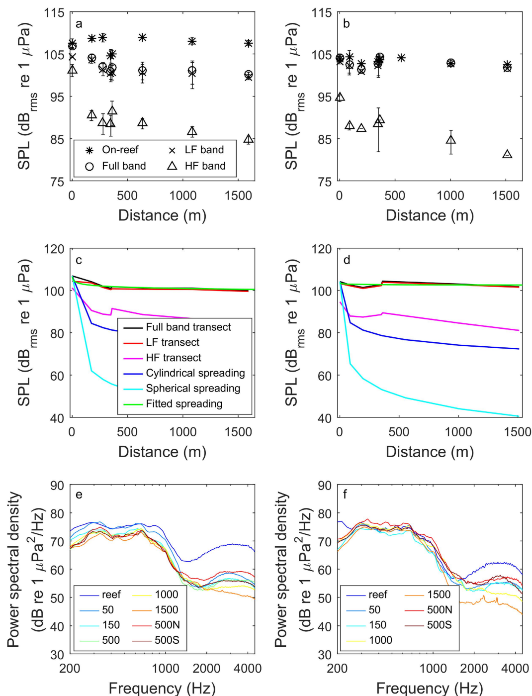
Figure 2. Mean ( \pm SD) sound pressure levels (200–4900 Hz) on the reef (full band) and low- (200–1000 Hz), high-frequency (2000–4000 Hz) and full-band SPL at various distances from the reef at dawn (a) and mid-morning (b). Transect levels for the full band, low- (LF) and high-frequency (HF) shown with estimated cylindrical and spherical spreading loss and full band fit lines (c,d) and associated mean power spectra for each distance from the reef at the two times of day (e,f). On-reef sound levels stayed relatively constant during the dawn transect and varied over time during the mid-morning transect; conversely, full-band transect levels decreased with distance from the reef during the dawn but not the mid-morning transect. While high-frequency SPL attenuated with distance from the reef at both times of day, levels were considerably lower than the low-frequency SPL and accordingly make less of a contribution to the full-band trends. In neither case did attenuation match predicted spreading loss. High frequencies were elevated on the reef compared to every other transect point and decreased rapidly with distance from the reef. Low frequencies during the dawn transect appeared to decrease with distance from the reef while no such trend was evident for the mid-morning transect. No data were retained for the 500 m position during the mid-morning transect. See Table 2 for the equations of the fit lines in (c,d).
