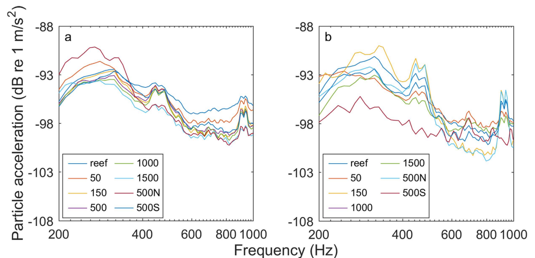
Figure 4. Mean particle acceleration values by transect, position, and frequency in the x-axis. Peaks in acceleration were seen below 500 Hz in both transects, but no clear pattern with distance was evident. Acceleration was elevated slightly at the 500 N position during the dawn transect (a) and at the 150 m position during the mid-morning transect (b). No data were available for the 500 m position during the mid-morning transect.
