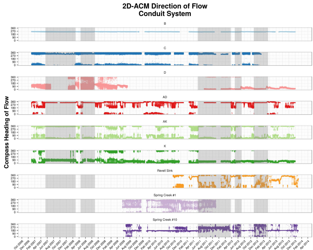
Figure 3. 2D-ACM direction of flow data for the Wakulla and Spring Creek conduit systems. Note that the y-axis, representing the compass heading of flow, is topologically discontinuous, and that the bottom of the graph (0 degrees) and top of the graph (360 degrees) both represent northward-flow.
