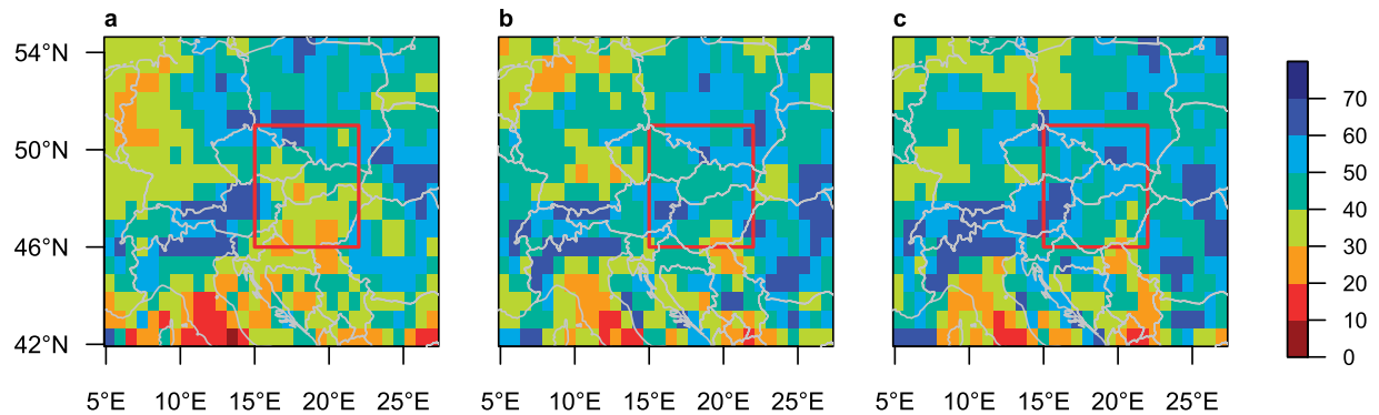
Figure 2. 20-summer return levels in model experiments. 20-season return level (RL20S) for JJA ( \text{mm}\cdot\text{d}^{-1} ) in (a) control, (b) Med warm , and (c) Glob warm . Red box denotes study region for area average and further analyses ( 15\text{--}22^\circ\text{E} , 46\text{--}51^\circ\text{N} ). Maps created with R version 3.2.3 ( www.r-project.org ).
