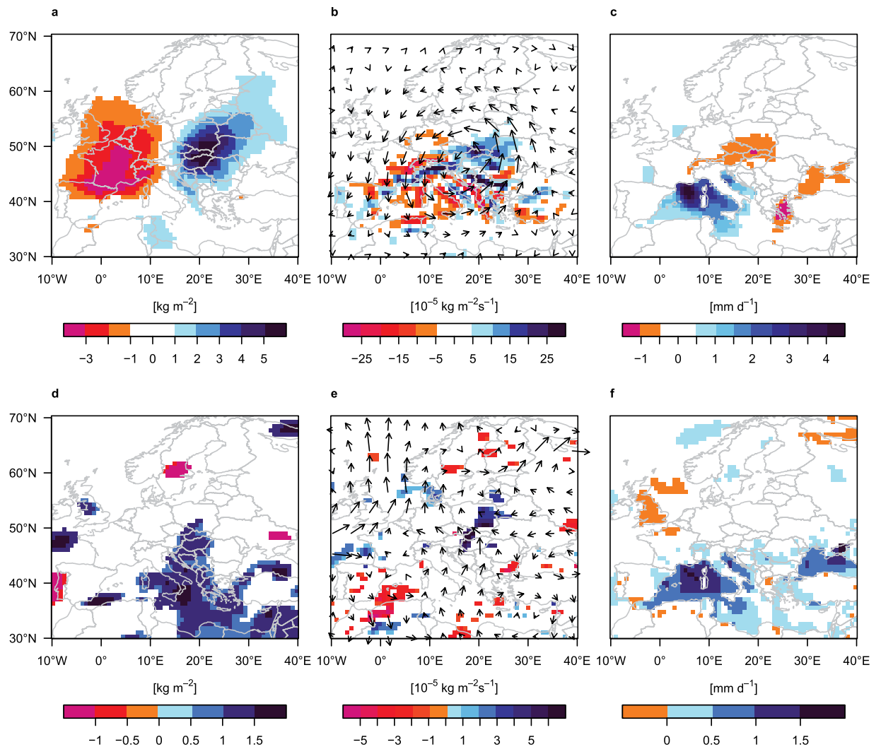
Figure 5. Variables related to the hydrometeorological cycle during heavy-precipitation events. Heavy-precipitation events are days where daily precipitation aggregated over the study region (15–22°E, 46–51°N; red box in Fig. 2) exceeds the 95th percentile of all summer days in the respective experiment. (a–c) Composite anomalies in control experiment (relative to climatology) and (d–f) significant differences (based on a two-sided independent samples t-test at the 90% significance level) between composites in Med warm and control: (a,d) Column integrated precipitable water ( \text{kg m}^{-2} ); (b,e) vertically integrated moisture convergence ( 10^{-5} \text{ kg m}^{-2} \text{ s}^{-1} ) and vertically integrated moisture transport as vectors (every fifth vector is plotted), vector length is (b) 50 \text{ kg m}^{-1} \text{ s}^{-1} per degree lon/lat and (e) 10 \text{ kg m}^{-1} \text{ s}^{-1} per degree lon/lat; (c,f) evaporation ( \text{mm d}^{-1} ). Maps created with R version 3.2.3 ( www.r-project.org ).
