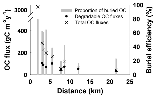
Fig. 4. Flux of degraded • and total x organic carbon (OC) together with burial efficiency as a function of distance from the Rhône River outlet.
