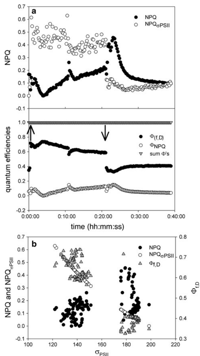
Fig. 7 Analysis of quenching yields subjected to a block light treatment (data Fig. 2). a Top panel NPQ calculated using the Stern–Volmer equation ( (F_m - F_m')/F_m' ), and as \text{NPQ}_{\sigma_{\text{PSII}}} ( (\sigma_{\text{PSII}} - \sigma_{\text{PSII}}')/\sigma_{\text{PSII}}' ). Bottom panel regulated NPQ ( \Phi_{\text{NPQ}} ) and constitutive NPQ plus fluorescence ( \Phi_{f,D} ) and the sum of all quantum efficiencies ( \Phi_{\text{NPQ}} + \Phi_{f,D} + \Delta F/F_m' ). b Relationship between \sigma_{\text{PSII}} (bottom X-axis) and the two proxies for the NPQ (left Y-axis) or the quantum efficiency for constitutive NPQ (right Y-axis). As can be seen there is an excellent relationship between changes in \sigma_{\text{PSII}} and \Phi_{f,D} , but not between changes in \sigma_{\text{PSII}} and changes in the “classical” NPQ
