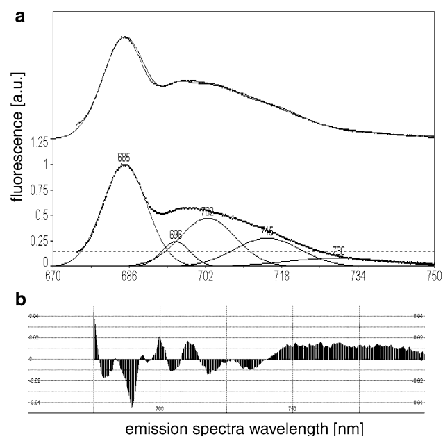
Fig. 4 Representative fluorescence emission spectrum measured at 77 K (a) and residuals remaining after de-convolution (b). A minimum of three measurements per sample were averaged and baseline corrected. The fit was forced through peaks at 685 nm (light harvesting compounds of PSII), 695 nm (PSII reaction core), 702 nm (origin not clear), 715 nm (PSI) and 730 nm (PSI, or vibration). Top curve: dots data points, line resulting fit from de-convolution. Although the origin of the F_{702} is obscure, leaving it out resulted in poor fits. Spectra were normalised to F_{658} nm. Residuals (b) show the quality of the fit and remained below 0.05 for all samples analysed. Emission peak height data were used for PSII/PSI ratio ( F_{685}/F_{715} nm). Excitation wavelength was 435 nm
