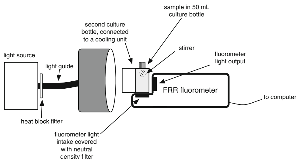
Fig. 1 Schematic drawing of the FRRF experimental set-up. A 50-ml culture bottle contained the samples and was placed against the FRR fluorometer so that it received the flashlet sequences from behind (fluorometer light output), and the actinic light the front (i.e. the left side in this drawing). The photomultiplier detected chlorophyll fluorescence from below. Due to relatively high cell densities, neutral
