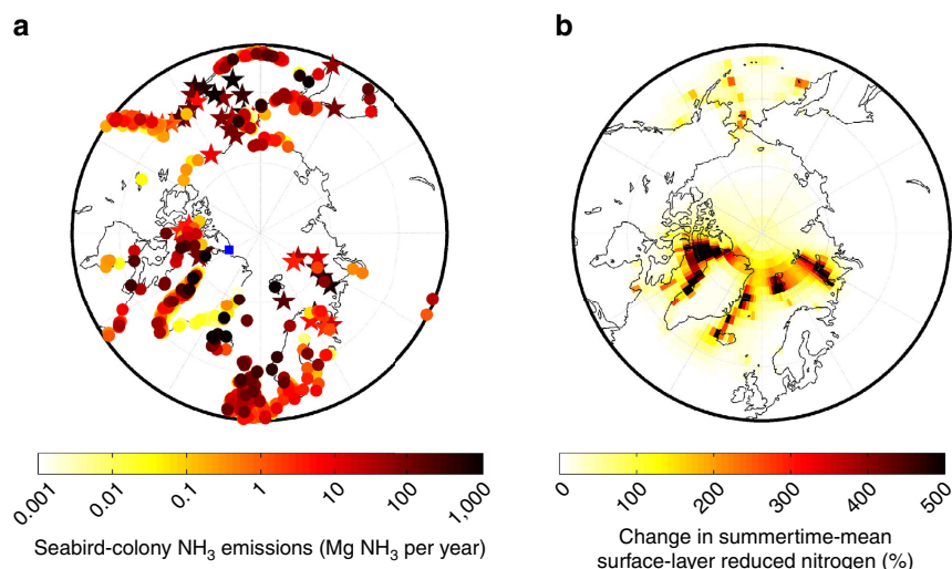
Figure 2 | Arctic seabird-colony \text{NH}_3 emissions and impacts on atmospheric surface-layer \text{NH}_3 and \text{NH}_4^+ mixing ratios. (a) Locations and annual emissions of \text{NH}_3 from Arctic seabird colonies. Circles indicate colonies in the Riddick et al. 18,19 inventory and stars are additional colonies from the Circumpolar Seabird Data Portal 30 . The blue square shows the location of Alert, Nunavut, Canada. (b) Percent change in summertime mean atmospheric surface-layer total reduced nitrogen (gas-phase ammonia ( \text{NH}_3 ) and particulate ammonium ( \text{NH}_4^+ )) attributed to the seabird-colony \text{NH}_3 emissions for the GEOS-Chem-TOMAS simulations.
