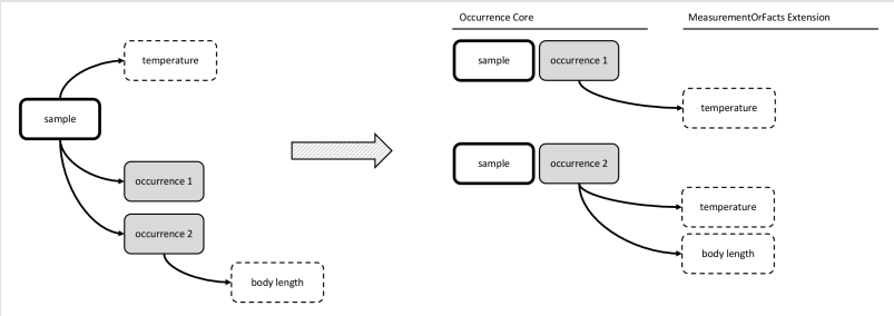
Figure 2. A schematic diagram of Option 1: Occurrence Core combined with MoF Extension. The diagram shows that the temperature measurement is duplicated in the MoF Extension for each occurrence record of the same sample.
