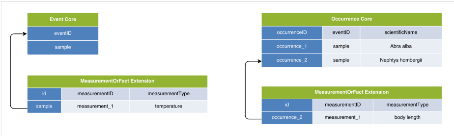
Figure 7. A practical example of Option 3: Event Core combined with MoF Extension & Occurrence Core combined with MoF Extension. This approach combines the best features of Option 1 and Option 2, but has the downside of separating the abiotic from the biotic data into different resources.
