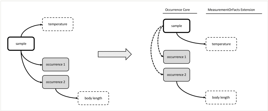
Figure 8. A schematic diagram of Option 4: Occurrence Core combined with MoF Extension; each sampling event is documented as a separate record in the Occurrence Core. The diagram shows that this format allows efficient storage of both biotic and abiotic measurements in the same DwC-A, but it increases complexity by introducing an event record without associated occurrence information into the Occurrence Core.
