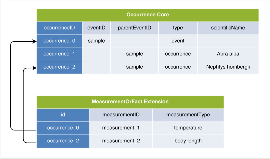
Figure 9. A practical example of Option 4: Occurrence Core combined with MoF Extension; each sampling event is documented as a separate record in the Occurrence Core. This example demonstrates that this format allows efficient storage of both biotic and abiotic measurements in the same DwC-A, but it increases complexity by introducing an event record without associated occurrence information into the Occurrence Core.
