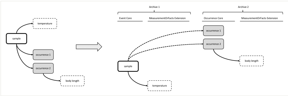
Figure 6. A schematic diagram of Option 3: Event Core combined with MoF Extension & Occurrence Core combined with MoF Extension. The diagram shows that this approach combines the best features of Option 1 and Option 2, but has the downside of separating the abiotic from the biotic data into different resources.
