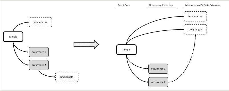
Figure 13. A schematic diagram of Option 6: Event Core combined with Occurrence Extension and a newly proposed MoF Extension; both extensions are linked with an OccurrenceID. The diagram shows that this is the most simple option to efficiently store both biotic and abiotic measurements in the same DwC-A.
