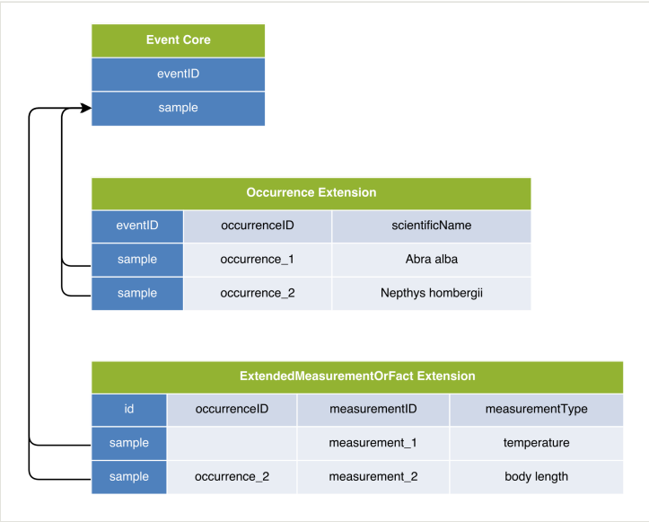
Figure 14. A practical example of Option 6: Event Core combined with Occurrence Extension and a newly proposed eMoF Extension; both extensions are linked with an OccurrenceID. This format is the most simple option to efficiently store both biotic and abiotic measurements in the same DwC-A.
