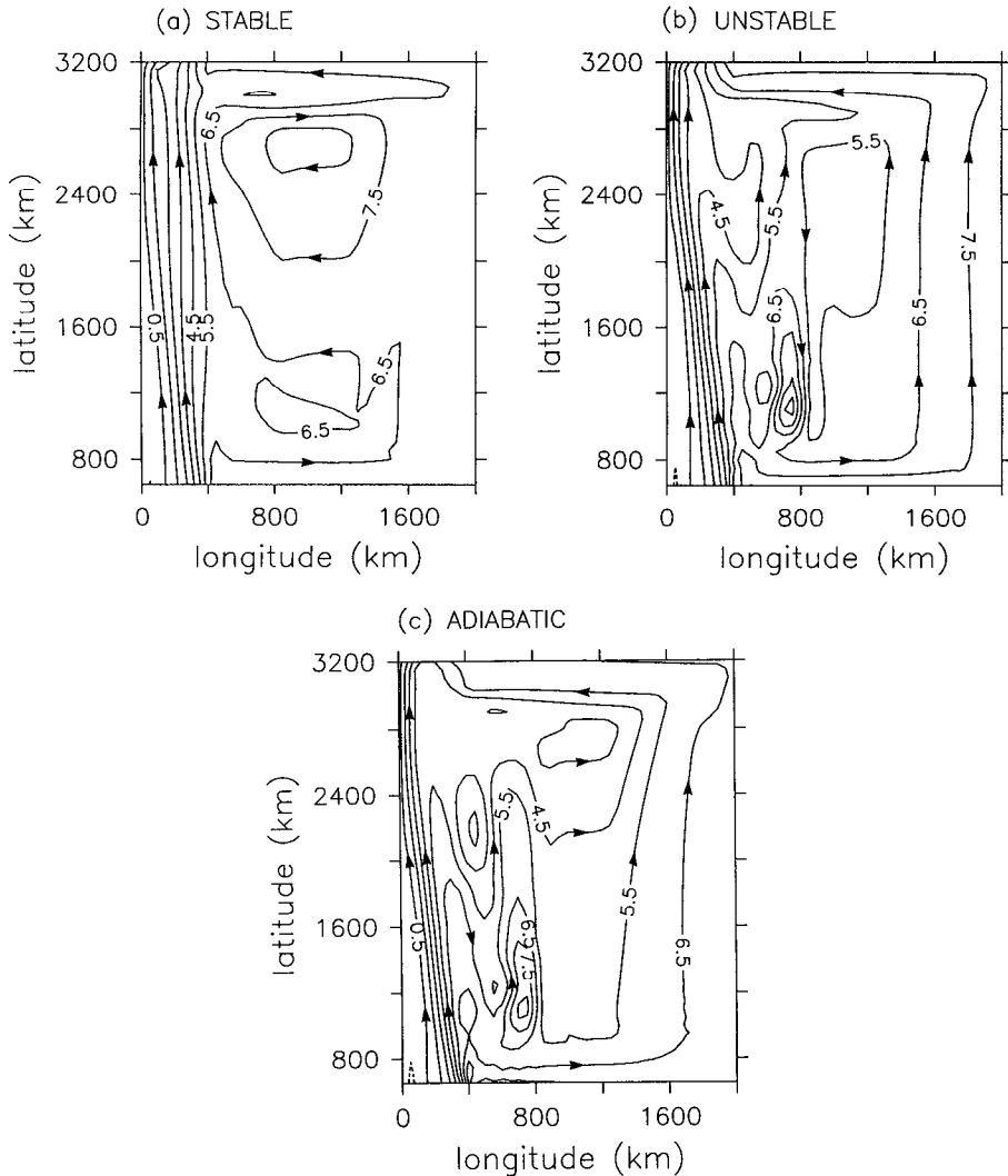
Figure 2. Mean transport streamfunction ( S_v ) for layers 2 + 3. (a) STABLE, stable western boundary current ( C_D = 0.03 ) with cross-isopycnal mixing, (b) UNSTABLE, unstable western boundary current ( C_D = 0.003 ) with cross-isopycnal mixing, (c) ADIABATIC, unstable western boundary current ( C_D = 0.003 ) with no cross-isopycnal mixing.
