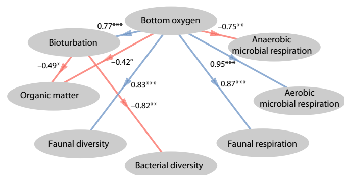
Fig. 4. Path diagram for the final model examining causal effects between bottom-water oxygen concentration (exogenous variable) and the endogenous variables: Organic matter ( C_{org} , chlorophyll a , and THAA), bioturbation, macrofaunal and meiofaunal diversity (based on inverse Simpson index), faunal and microbial aerobic and anaerobic respiration [from Lichtschlag et al. (37)], and bacterial diversity (based on inverse Simpson index from ARISA). Arrows (paths) indicate negative (red) or positive (blue) effects of bottom-water oxygen concentration, respectively, and numbers associated with arrows represent path coefficients. The goodness-of-fit index of the model was 0.75. * P < 0.05 ; ** P < 0.01 ; *** P < 0.001 . ° P = 0.08 , marginally significant trend.
