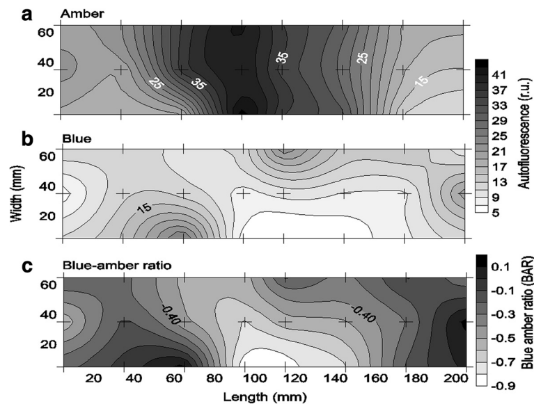
Fig. 2 Spatial distribution of autofluorescence (relative units) distribution in the photosynthetic microbial mat on Schiermonnikoog in November 2012, after a amber (cyanobacteria) light exposure, b blue (diatoms) light exposure, and c blue to amber ratio (BAR). Area of studied sample: 210 × 70 × 1 mm (L × W × H). Crosses indicate sampling points
