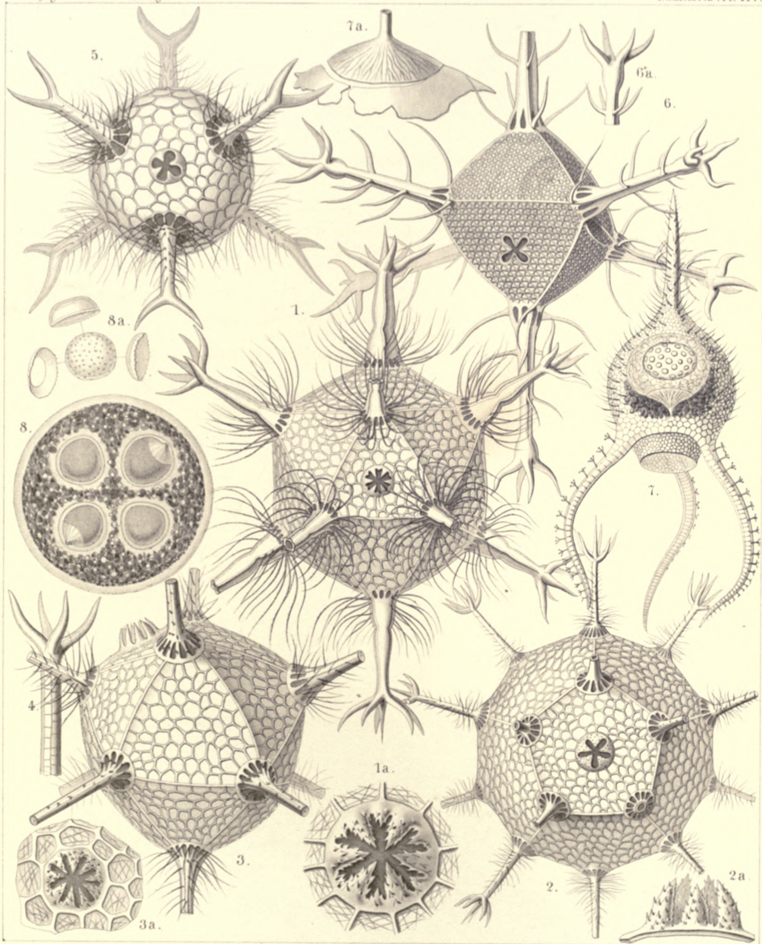
1. CIRCAGONIA . 2. CIRCORRHEGMA . 3. CIRCOSPAPHIS . 4-6. CIRCOPORUS , 7. CORTINETTA , 8. CATINULUS .
