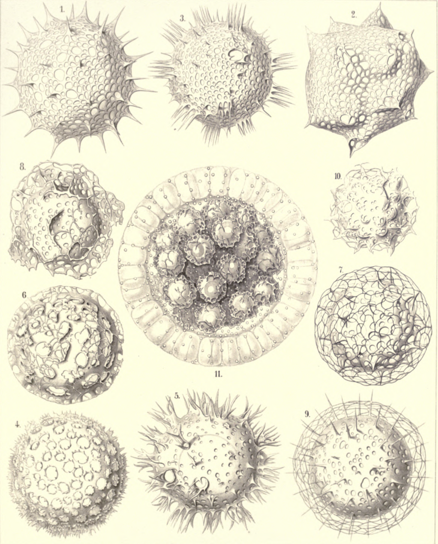
1. 2. ACROSPHAERA, 3-5. CHOENICOSPHAERA, 6-8. CLATHROSPHAERA, 9-11. XANTHIOSPHAERA.
