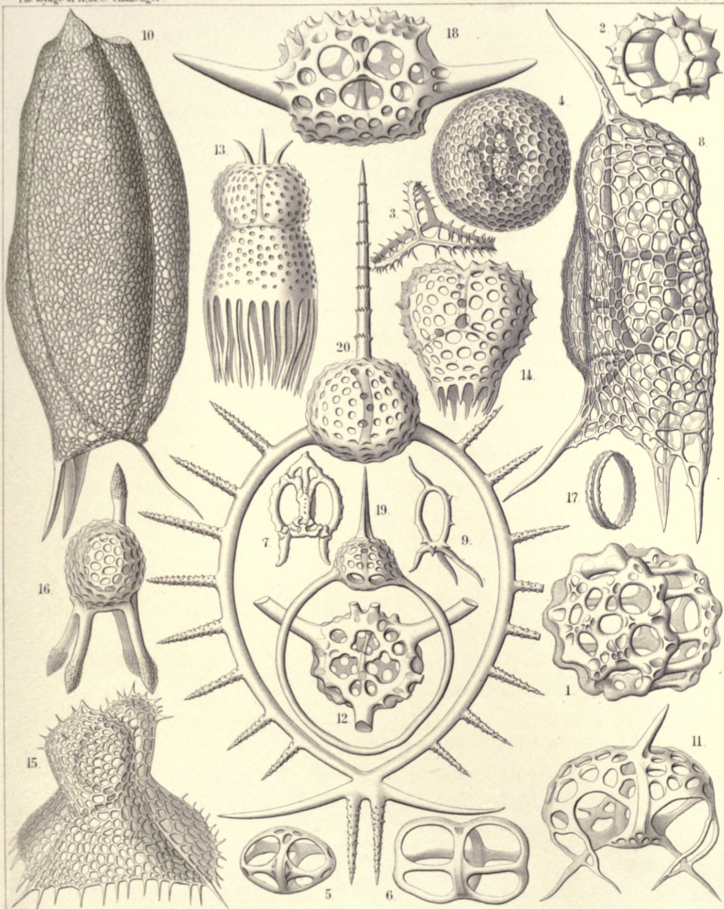
1. 2. LITHOTYMPANIUM, 3. DYOSTEPHANUS, 4. SPHAEROCIRCUS, 5. 6. TRISSOCYCLUS, 7. DIPOCORONIS, 8. - 10. LAMPROSPYRIS, 11. 12. CLADOSPYRIS, 13. RHODOSPYRIS, 14. 15. DESMOSPYRIS, 16. 17. TETRASPYRIS, 18. - 20. STEPHANOSPYRIS.
