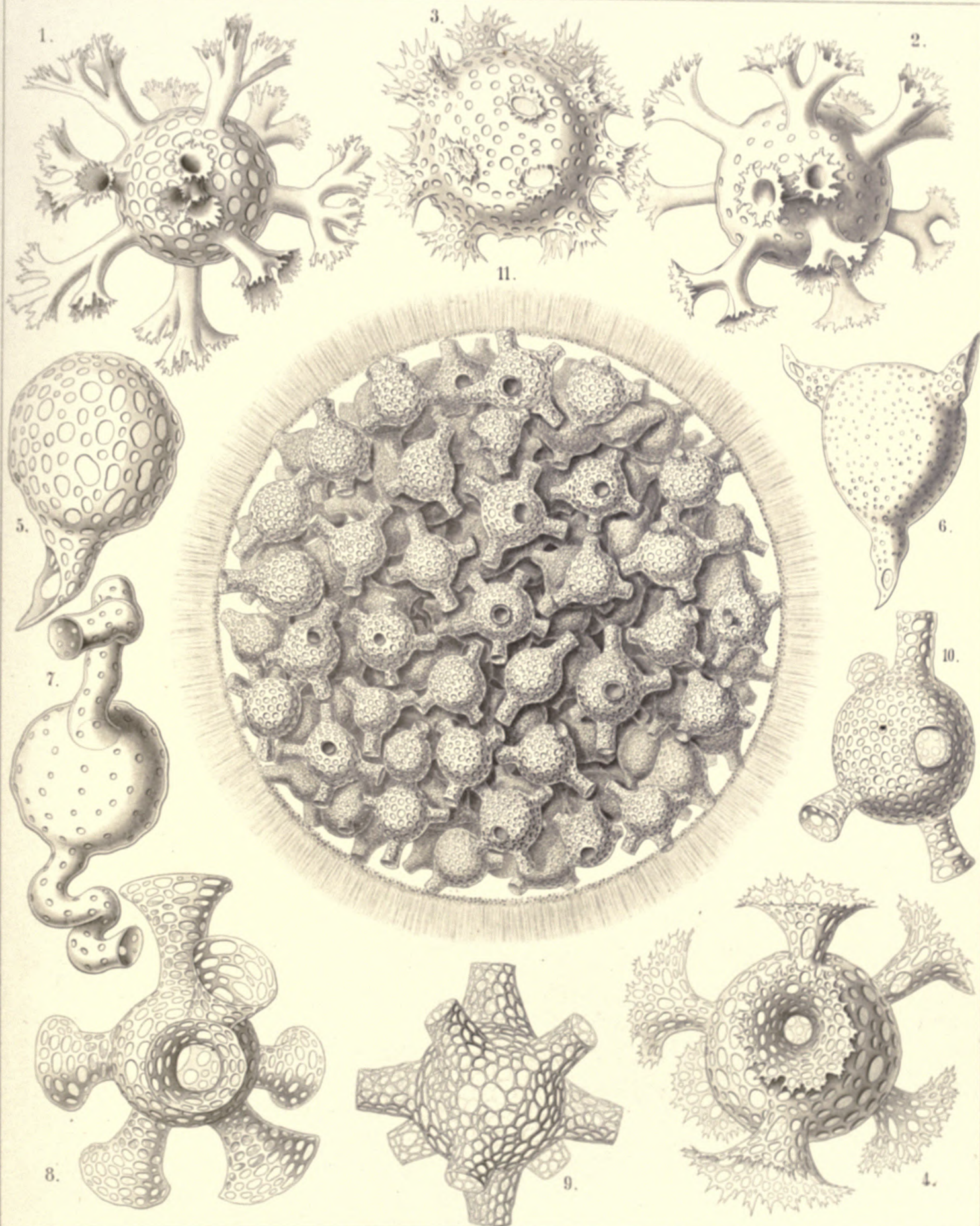
1, 2. CAMINOSPHERA, 3, 4. CORONOSPHERA, 5, 6. OTOSPHERA, 7-11. SOLENOSPHERA.
