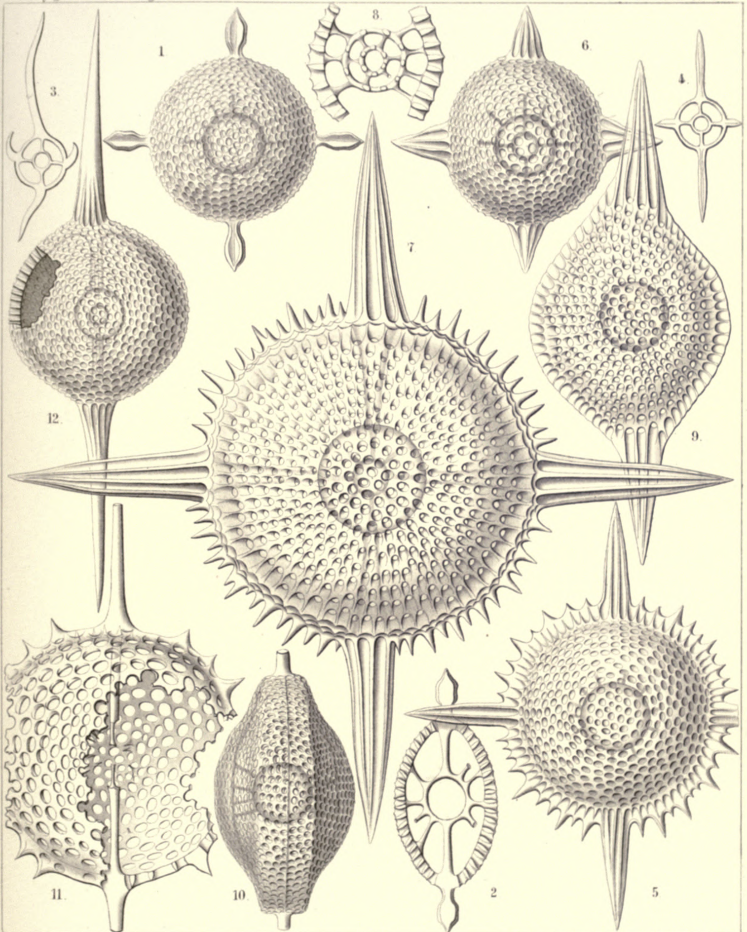
1-4. SETHOSTAURUS, 5. HELIOSTHAURUS, 6. PHACOSTHAURUS, 7, 8. ASTROSTHAURUS, 9-11. SETHOSTYLUS, 12. PHACOSTYLUS.
