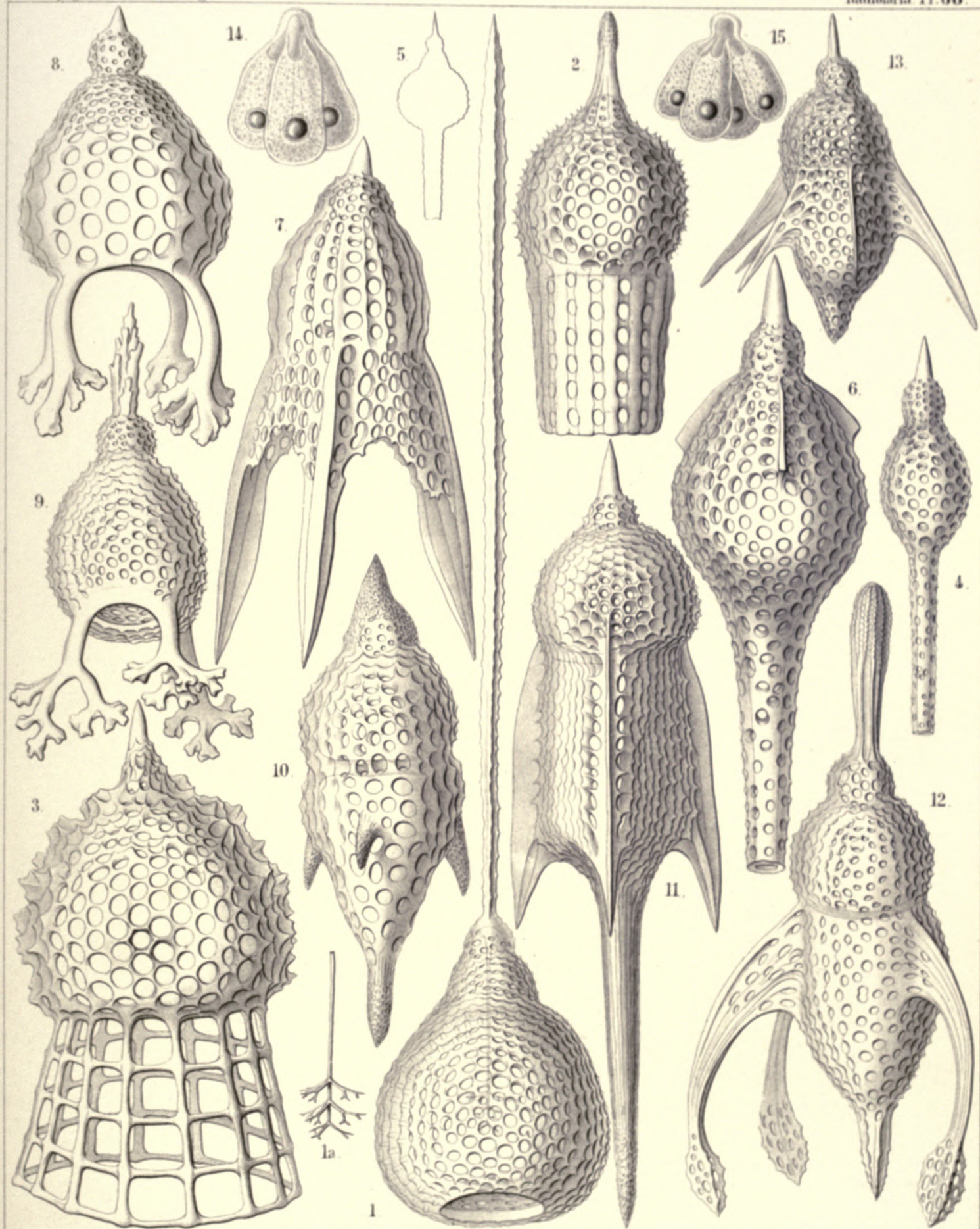
1. AXOCORYS, 2. 3. CYCLADOPHORA, 4. 5. THEOSYRINGIUM, 6. PTEROSYRINGIUM, 7. PTEROCANIUM, 8. 9. THYRSOCYRTIS, 10. 11. RHOPALATRACTUS, 12. DICTYATRACTUS, 13. HEXALATRACTUS.
