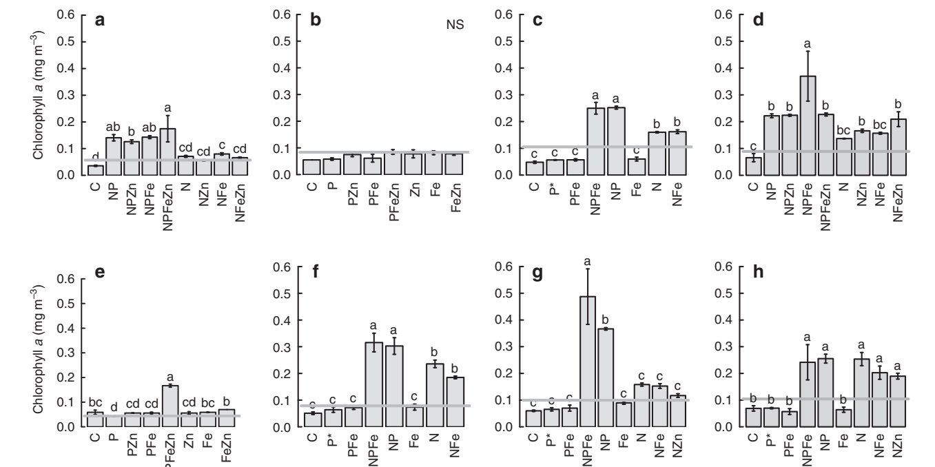
Figure 3 | Chlorophyll a responses to nutrient additions. (a–h) Experiments 1–8. Shown are means ± s.e.'s, n = 3 for all except where indicated by an asterisk ( n = 2). The grey horizontal line is the mean initial time point measurement ( n = 3). Treatment means were compared using a one-way analysis of variance and a Fisher PLSD means comparison test (indistinguishable means labelled with the same letter ( P < 0.05); NS is 'not significant').
