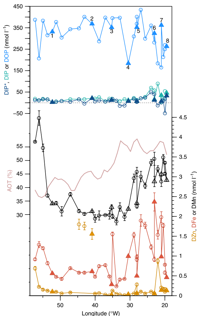
Figure 2 | Cross-Atlantic nutrient trends. DIP = dissolved inorganic phosphorus, DIP* represents excess available DIP based on a 16:1 N:P requirement of phytoplankton ( = \text{DIP} - \text{DIN}/16 ; DIN is dissolved inorganic nitrogen), DOP = dissolved organic phosphorus, DFe = dissolved Fe, DZn = dissolved zinc, and DMn = dissolved manganese, AOT = aerosol optical thickness (satellite-derived average for May 2015). Error bars on metal concentrations represent the s.d. calculated from the precision of the isotope ratios and counting of the mass spectrometer. Sampling locations are highlighted with black dots in Fig. 1a and filled triangles indicate concentrations measured at experiment start points. High dissolved Zn concentrations around 40–45 °W indicate potential trace Zn contamination of these three samples.
