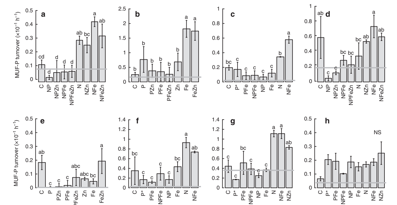
Figure 4 | Alkaline phosphatase activity responses to nutrient additions. (a–h) Experiments 1–8. Activities are shown as turnover rates of the spiked DOP substrate, 4-methylumbelliferyl phosphate (MUF-P). Shown are means ± s.e.'s, n = 3 for all except where indicated by an asterisk ( n = 2). The grey horizontal line is the mean initial time point measurement ( n = 3). Treatment means were compared using a one-way ANOVA and a Fisher PLSD means comparison test (indistinguishable means labelled with the same letter ( P < 0.05); NS is 'not significant').
