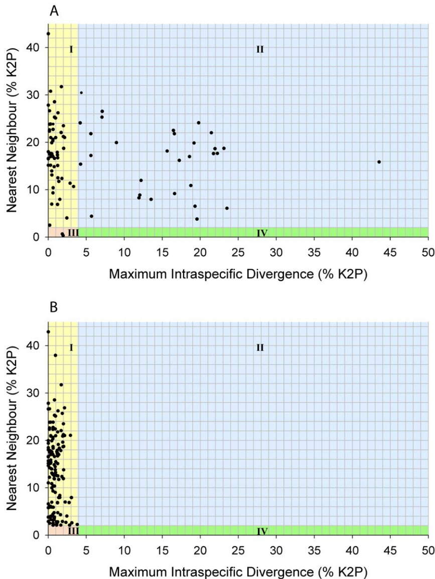
Figure 3. Comparison of COI (K2P) distances between morphologically identified polychaete species (A) and MOTUs (B). Plotting axes at 2% nearest neighbour divergence (y-axis) and 10\times the average intracluster divergence of 3.8% (x-axis) creates four species categories where intraspecific distance and nearest neighbour distance respectively are: I) <3.8\% , >2\% : typical species; II) >3.8\% , >2\% : probable species complex; III) <3.8\% , <2\% : hybridization, young species, synonymy; IV) >3.8\% , <2\% : possible specimen misidentification. doi:10.1371/journal.pone.0022232.g003
