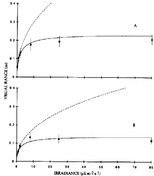
Fig. 2. Observed ( \pm 1 std. dev.) and modelled visual range in Gobiusculus flavescens as a function of light intensity and prey (A: Calanus finmarchicus , B: Acartia longiremis ). Solid line represents model with saturation (Eq. 8, T_1 = 7.5 \cdot 10^{-2} and 11.6 \cdot 10^{-2} for C. finmarchicus and A. longiremis respectively, K_e = 5 \mu E m^{-2} s^{-1} for both prey), while broken line represent the model of AKSNES and GISKE (1993) without saturation (Eq. 3).
