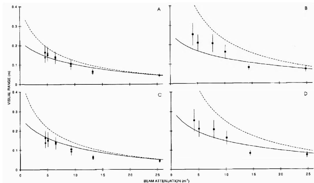
Fig. 3. Observed ( \pm 1 std. dev.) and modelled visual range in Gobiusculus flavescens as a function of beam attenuation with C. finmarchicus as prey (A,C: at light intensity 12 \mu\text{E m}^{-2} \text{s}^{-1} B,D: at light intensity 120 \mu\text{E m}^{-2} \text{s}^{-1} ). Solid line represents the model with saturation (Eq. 8), while broken line represents the model of AKSNES & GISKE (1993) without saturation (Eq. 3). In A and B we have used the same parameter set as in Fig. 2 ( T_1 = 7.5 \cdot 10^{-2} , K_e = 5 \mu\text{E m}^{-2} \text{s}^{-1} ), while C and D show the effect of increasing the inherent prey contrast with 50 % (see text for discussion). The different symbols in A and C represents results from two independent experiments.
