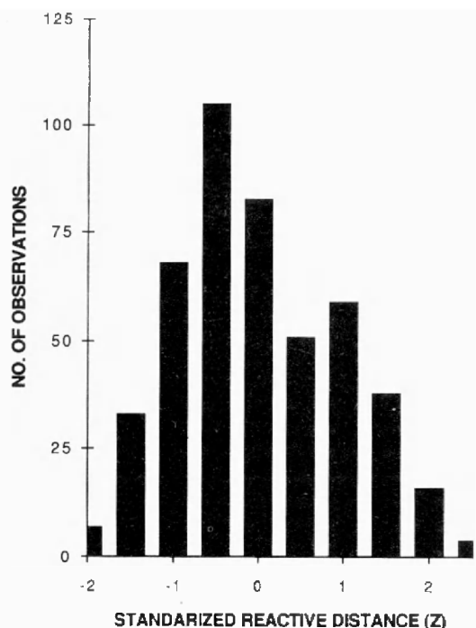
Fig. 1. The standardised distribution of 480 reactive distance measurements in Gobiusculus flavescens with Calanus finmarchicus as prey item (UTNE 1997). The individual reactive distance measurements were standardised according to z = (x - R) / s where x is the reactive distance, R is the mean reactive distance for one experimental set-up and s is the standard deviation. The visual range ( r_0 ) was defined as R + 2s , which corresponds to a standardised reactive distance, z = 2 .
