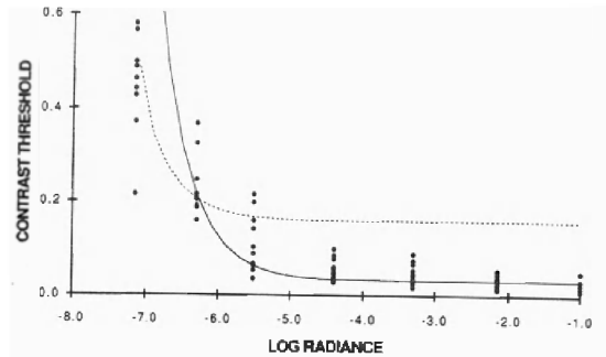
Fig. 5. The modelled versus the measured contrast threshold of Gadus morhua (ANTHONY 1981). The solid line was obtained with the parameter values T_3 = 3.19 \cdot 10^{-2} and K_e = 2.9 \cdot 10^{-6} \text{ W m}^{-2} \text{sr}^{-1} . Broken line indicates the result of increased contrast sensitivity (by lowering T_3 and K_e ) at low irradiance levels. Observations are redrawn from Fig. 5 in ANTHONY (1981).
