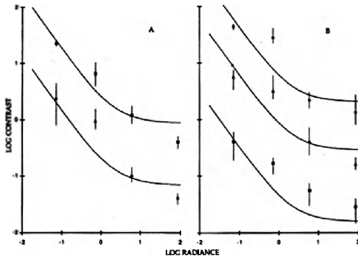
Fig. 4. The modelled (solid line) versus the measured (mean with max. and min. observation) contrast threshold of Carassius auratus as (HESTER 1968). (A: size groups 26 (squares) and 92 (triangles) min. of arc, B: size groups 17 (circles), 45 (triangles) and 194 (squares) min. of arc). All modelled lines were generated by T_2 = 5.8 \cdot 10^2 and K_e = 2.0 \mu\text{W cm}^{-2} \text{sr}^{-1} . Observations are redrawn from Fig. 7 in HESTER (1968). Ranges indicate maximal and minimal observation.
