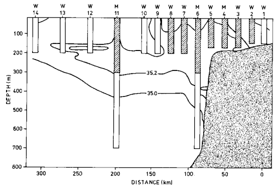
Fig. 2. Occurrence of Apolemia uvaria at the 14 stations along the Svinøy transect, based on WP2 samples (W, 200–0 m or bottom–0 m) and MOCNESS (M, eight sample intervals between 700 and 0 m). Shaded bars: Apolemia present; Open bars: Apolemia not present. The isohaline of 35.0 psu defines high salinity water of Atlantic origin.
