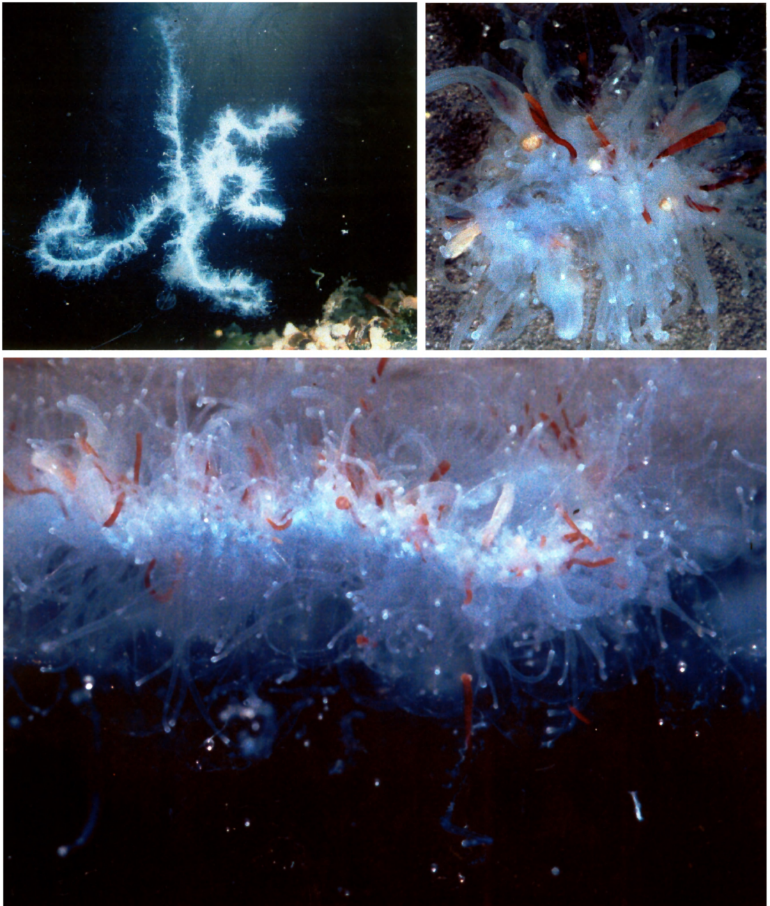
Fig. 3. Apolemia uvaria collected from the surface water. Top left: A whole colony with the stem contracted showing the typical irregular shape. Top right: Closer view of a cornidium group, clearly showing the two types of palpons (brownish and transparent) and a few gastrozooids. Bottom: A closer view of a section of the colony showing the typical appearance of a continuous mass of palpons and a few gastrozooids. All photos by Alf J. Nilsen.
