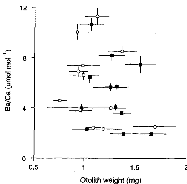
Fig. 7. Mean otolith Ba/Ca values ( \pm SE) from laboratory-reared Leiostomus xanthurus plotted against mean otolith weight ( \pm SE) for each of 24 rearing tanks maintained at either 20°C (■) or at 25°C (○).
