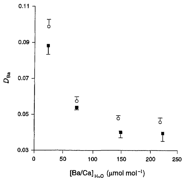
Fig. 5. Relation between estimates ( \pm \text{SE} ) of Ba partition coefficients ( D_{\text{Ba}} ) for otoliths of laboratory-reared Leiostomus xanthurus and Ba/Ca ratios of the rearing water ( [Ba/Ca]_{\text{H}_2\text{O}} ) at either 20°C (■) or at 25°C (○).
