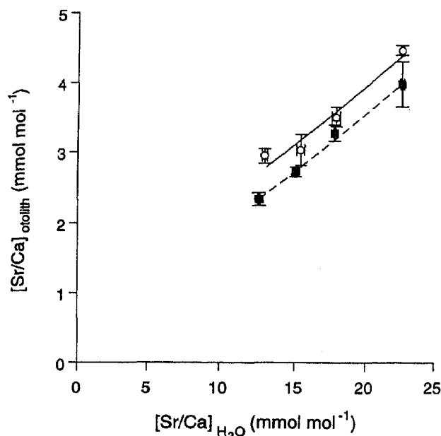
Fig. 3. Mean Sr/Ca ratios ( [Sr/Ca]_{\text{otolith}} \pm \text{SE} ) in otoliths of laboratory-reared Leiostomus xanthurus plotted against Sr/Ca ratios of the rearing water ( [Sr/Ca]_{\text{H}_2\text{O}} \pm \text{SE} ) at either 20°C (■, dashed line) or at 25°C (○, solid line). Lines were fitted by linear least-squares regression for each of the temperature treatments.
