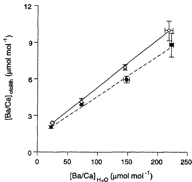
Fig. 4. Mean Ba/Ca ratios ( [Ba/Ca]_{\text{otolith}} \pm \text{SE} ) in otoliths of laboratory-reared Leiostomus xanthurus plotted against Ba/Ca ratios of the rearing water ( [Ba/Ca]_{\text{H}_2\text{O}} \pm \text{SE} ) at either 20°C (■, dashed line) or at 25°C (○, solid line). Lines were fitted by linear least-squares regression for each of the temperature treatments.
