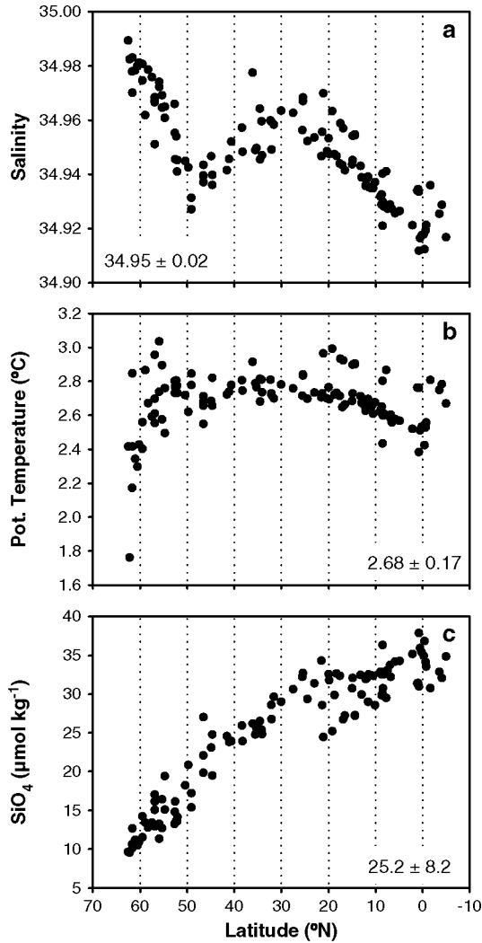
Figure 2. Observed latitudinal gradients of physicochemical parameters in the NEADW core. (a) Salinity, (b) potential temperature (°C), and (c) silicate ( \text{SiO}_4 ; \mu\text{mol kg}^{-1} ) along the transect from 70°N to 10°S. Numbers in the inset indicate average \pm standard deviation over the transect.
