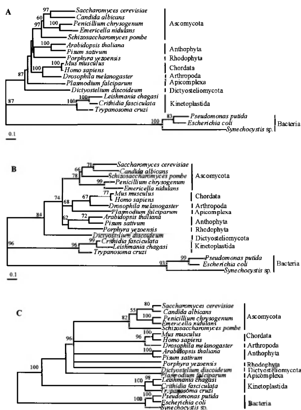
Fig. 3. Phylogenetic trees, which include Anthophyta, Apicomplexa, Arthropoda, Ascomycota, Bacteria, Chordata, Dictyosteliomycota, Kinetoplastida and Rhodophyta, based on the type II DNA topoisomerase amino acid sequences. Trees were artificially rooted on the branch leading to Bacteria. A: neighbour-joining tree. Distances were estimated using the Dayhoff PAM matrix. B: maximum likelihood tree. Model of amino acid substitutions was the JTT model. C: most parsimonious tree.
