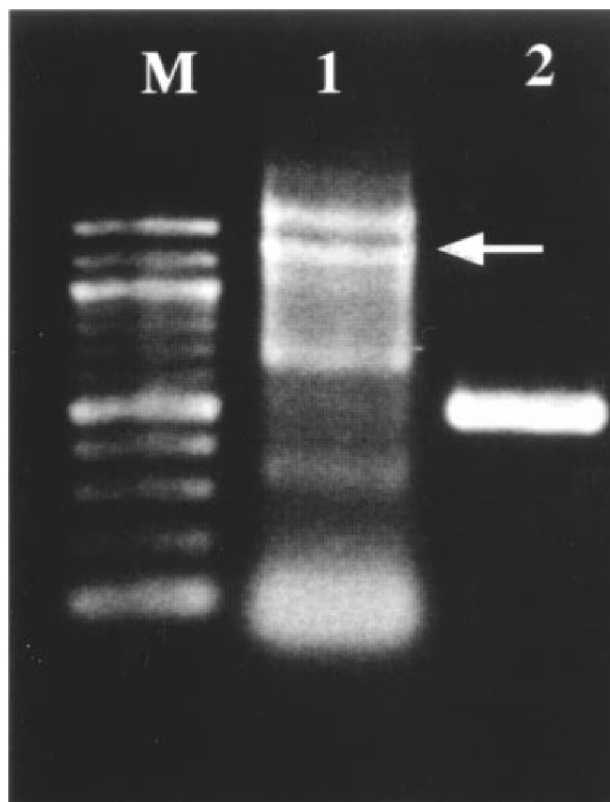
Fig. 1. Gel electrophoresis of PCR products amplified with degenerate primers (Primers A and B). Possible TOP2 is indicated as an arrow. Lane M, molecular size marker (100 bp DNA ladder); lane 1, amplified fragments of DNA of Porphyra yezoensis ; lane 2, positive control ( \lambda -DNA).
