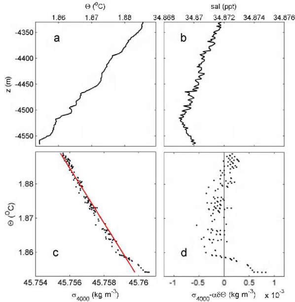
Figure 2. CTD observations just prior to deployment of the mooring, over the lower 220 m above the bottom: (a) conservative temperature, (b) salinity, (c) density anomaly (referenced to 4000 m)—Conservative temperature relationship, and (d) goodness of fit (dotted observations in plot Figure 2c—red line fit).
