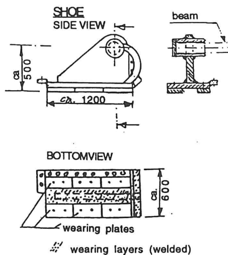
Fig. 3b. Gear-detail
