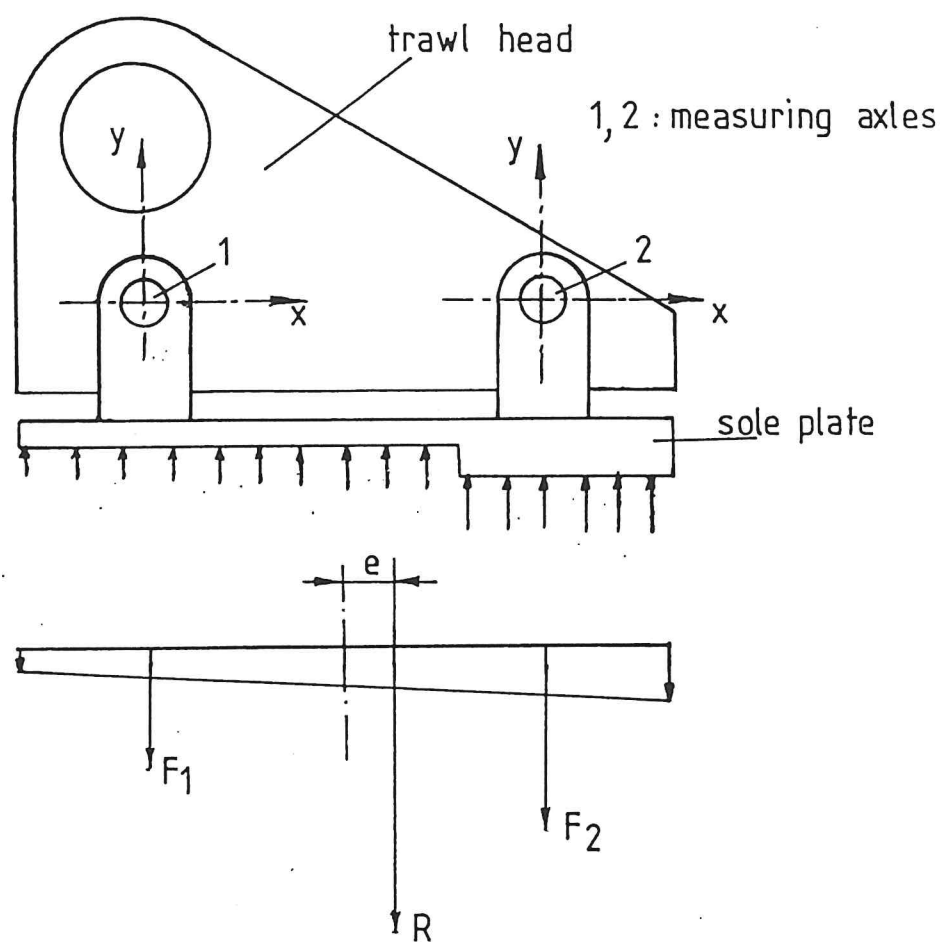
Fig. 3. Instrumented trawlhead-principle.
