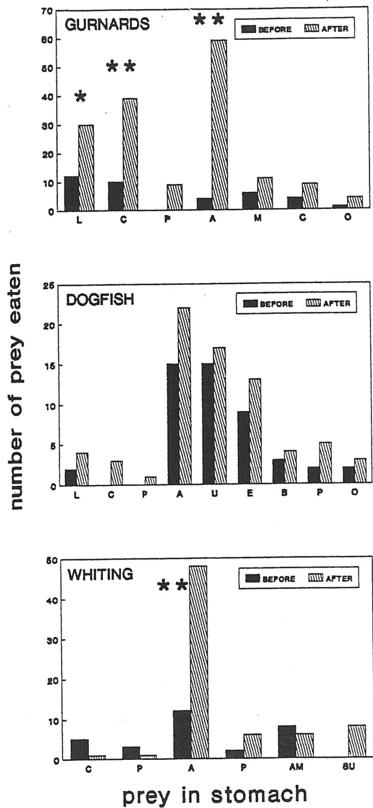
Fig. 4. The mean number of prey per stomach for gurnards, dogfish and whiting which were collected both before, and 3 h after fishing an area with a 4-m beam trawl. Significant differences were determined using the G-test (SOKAL & ROHLF, 1981), **= P < 0.05 , ***= P < 0.01 , ****= P < 0.001 .
