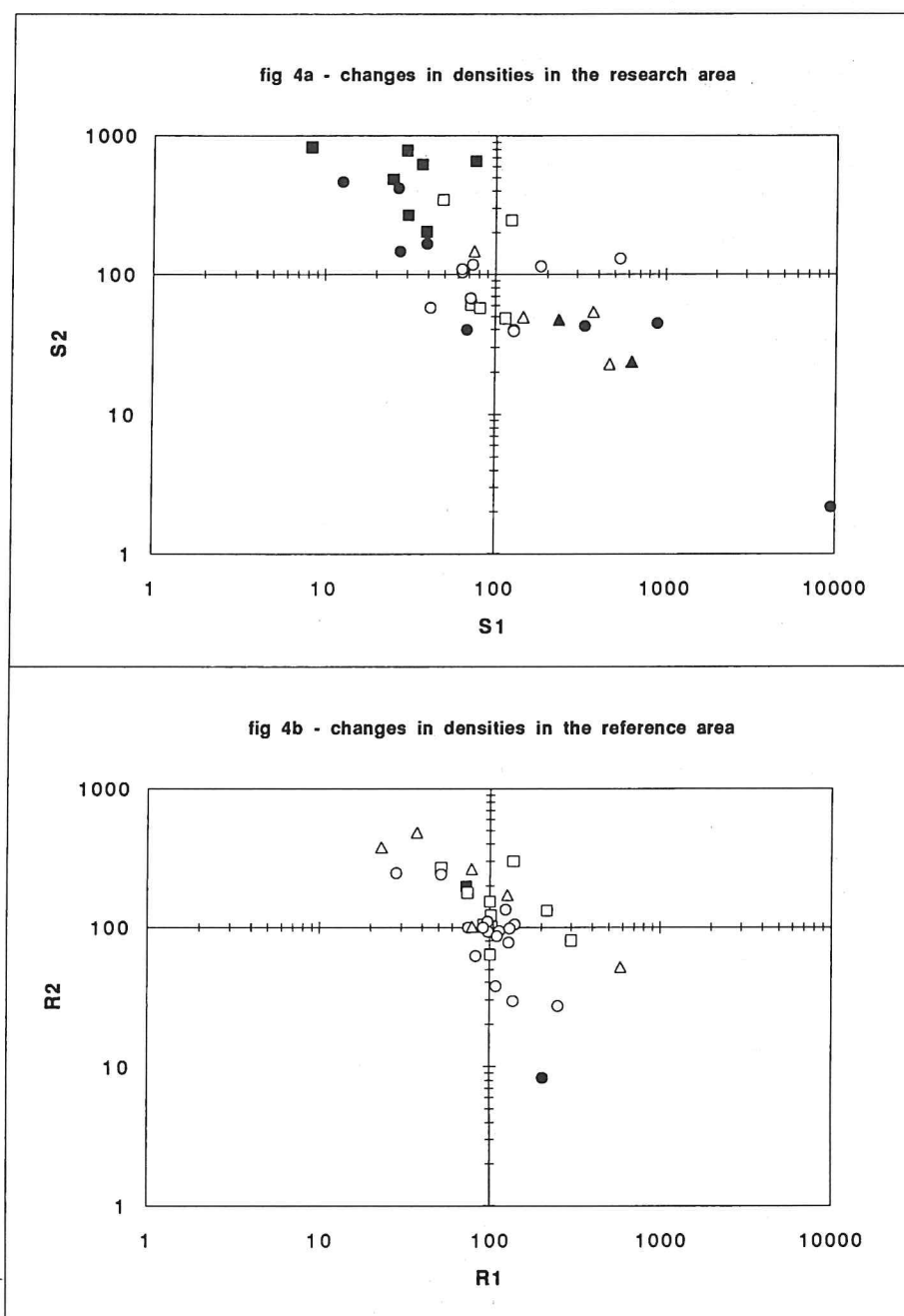
Fig. 4. Changes in density (%) in the study area between t_0 and t_1 ( S_1 = 100 \cdot t_1/t_0 ) and between t_1 and t_2 ( S_2 = 100 \cdot t_2/t_1 ), as well as in the reference area between t_0 and t_1 ( R_1 ) and between t_1 and t_2 ( R_2 ), of those species that were present in the three sampling periods in both area's (September study). Percentages >100\% denote an increase in density, percentages <100\% denote a decrease. M fish species; O mobile epi- and infauna; \Delta sedentary epi- and infauna; dark symbols indicate statistical significance of one or both changes in mean density.
