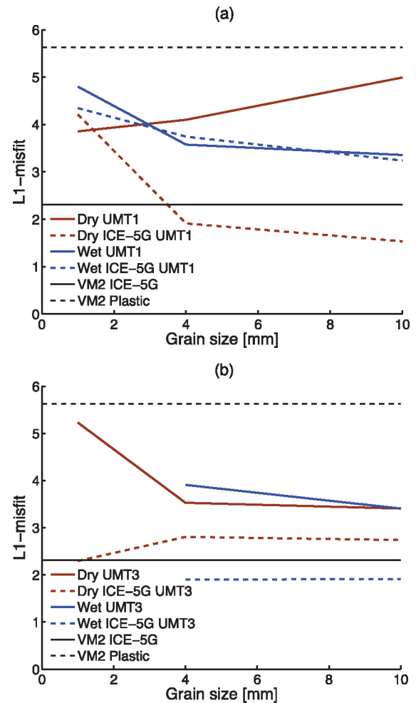
Figure 11. One-norm misfit for dry and wet rheology for the plastic ice model and ICE-5G. (a) UMT1 (upper-mantle temperatures derived from heatflow). (b) UMT3 (upper-mantle temperatures derived from seismic velocity anomalies).
