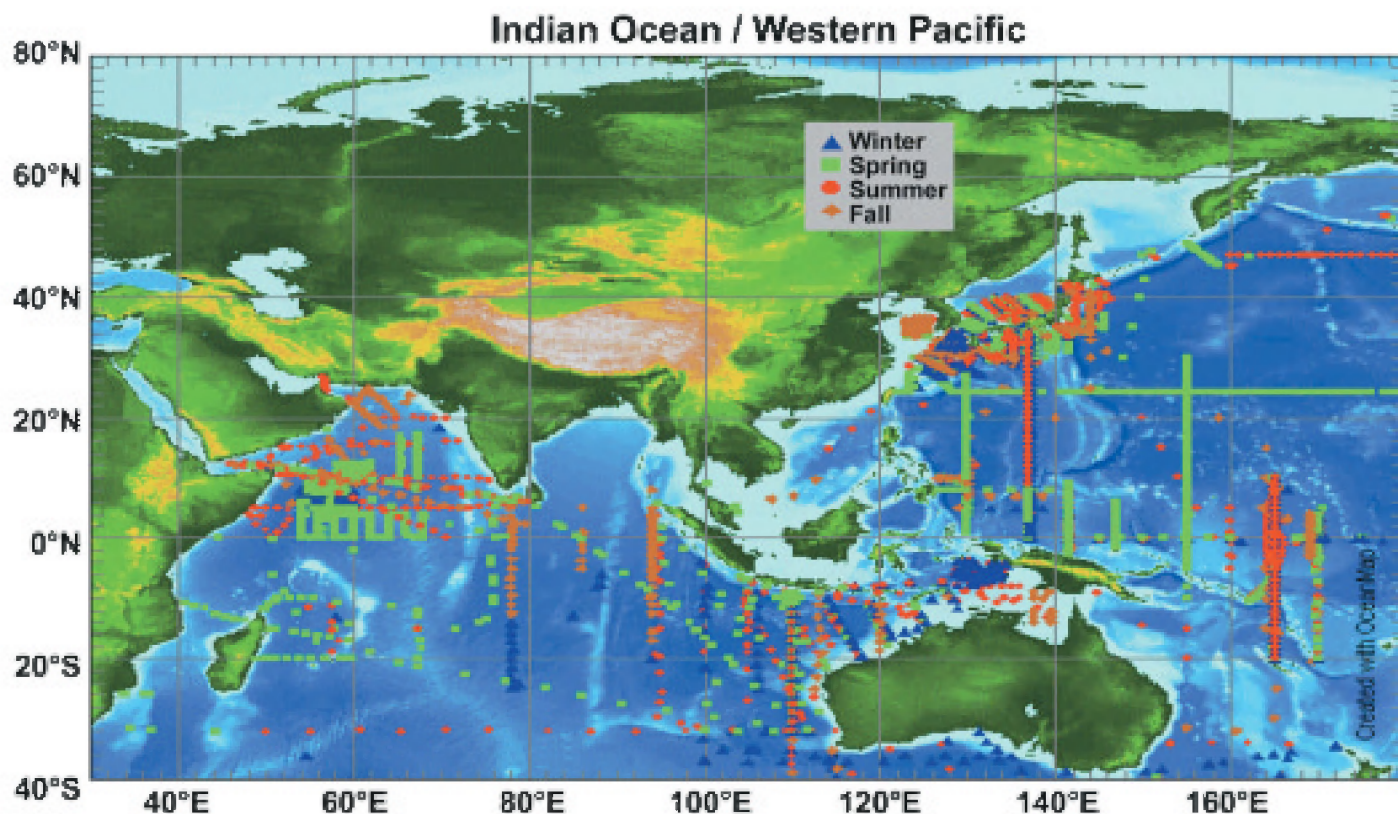
Figure 1. Example of WOOD K_d Locations in the Indian and Western Pacific Oceans.
