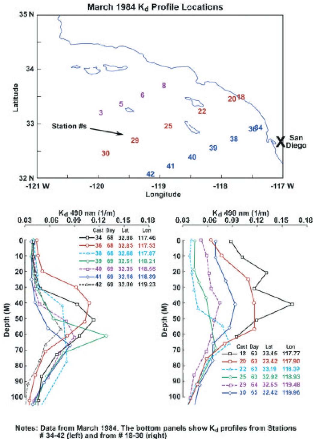
Figure 2. Example of WOOD used to assess spatial variability in K_d off Southern California.
