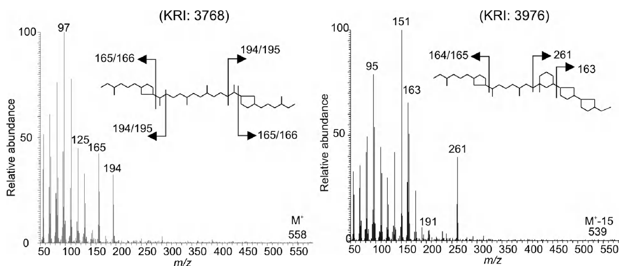
Figure 3. Mass spectra corresponding to biphytanes released from a prepared GDGT fraction enriched in GDGT-X after treatment with HI/LiAlH 4 . Kirchman Retention Indices (KRI) are indicated in brackets.
