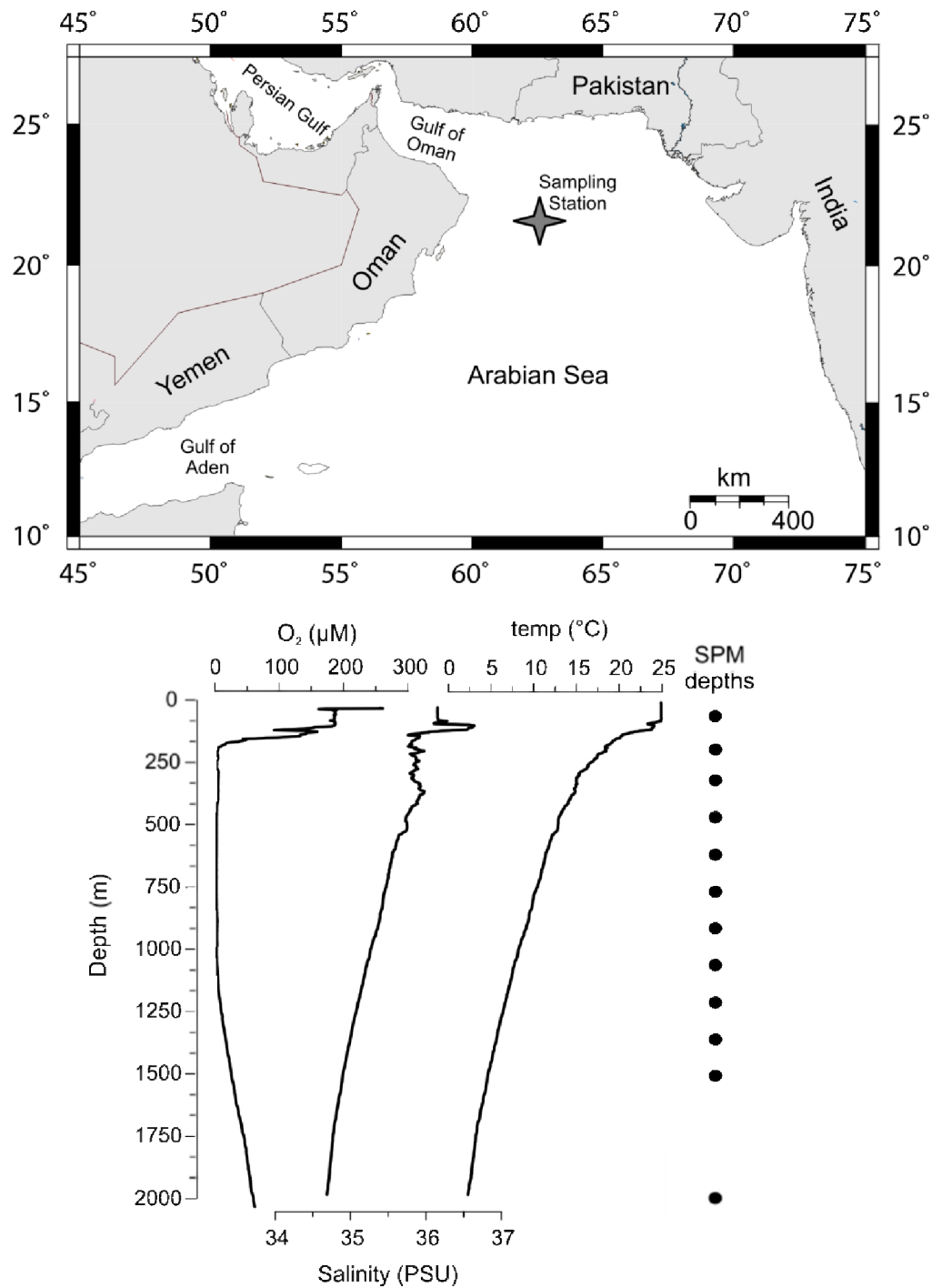
Figure 2. Location map and continuous CTD profile of oxygen, salinity and temperature (from Pitcher et al. (2010b)).
