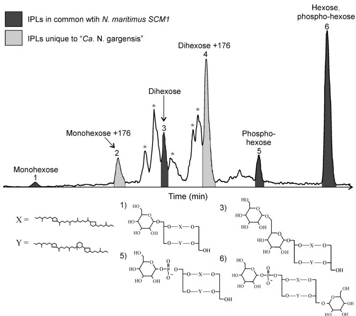
Figure 4. HPLC-ESI/MS base peak chromatogram of intact polar lipids extracted from " Ca. Nitrososphaera gargensis ". Numbered peaks correspond to structures described in Table 2 and tentative structures drawn below the chromatogram (with the exception of IPLs eluting in peaks 2 and 4, which were not drawn due to the unknown nature of the 176-
