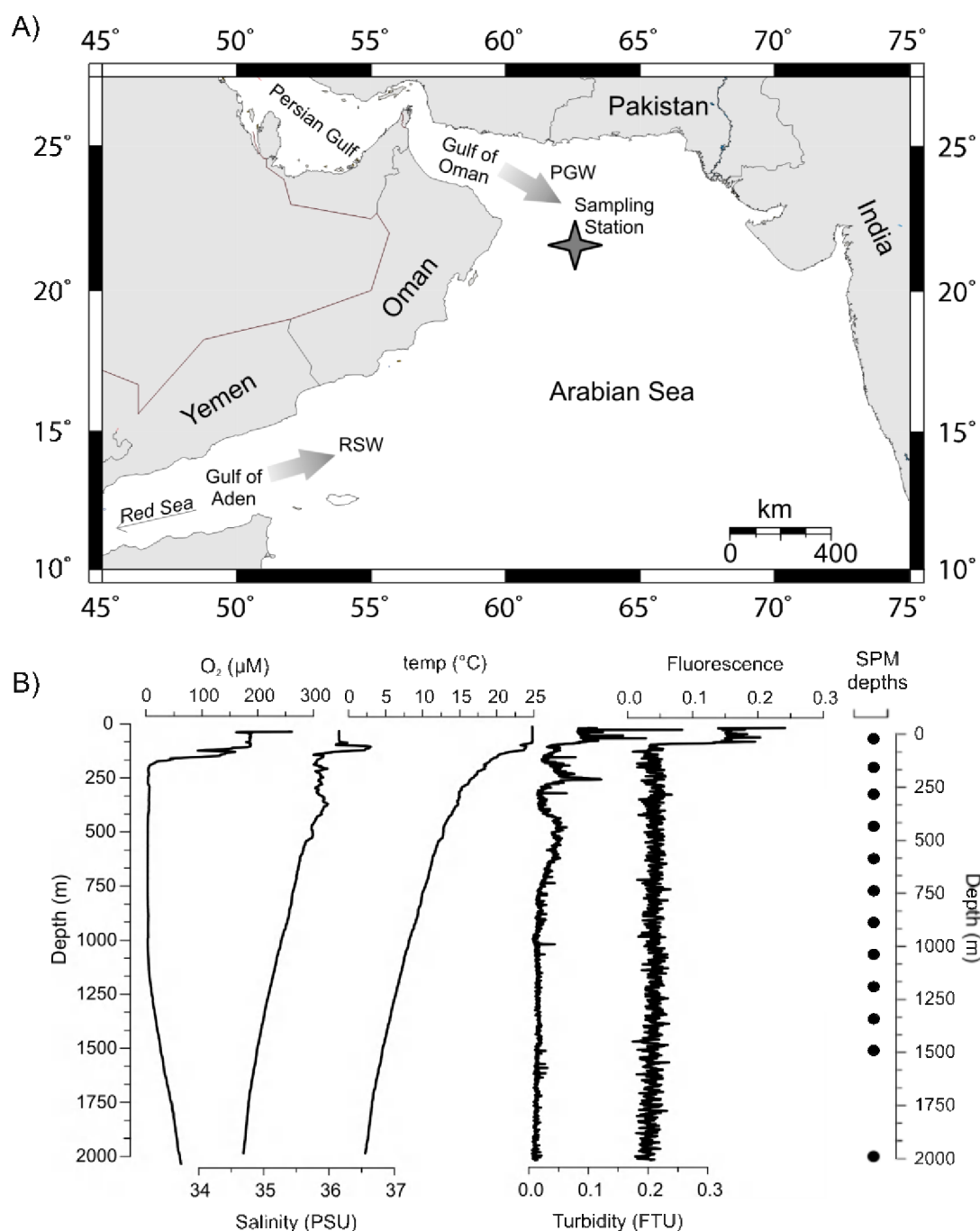
Figure 2. (A) Location of Arabian Sea sampling station (star; lat 21°55', long 63°10'). Persian Gulf Water (PGW) and to a much lesser extent, Red Sea Water (RSW), influence the oxygen minimum zone (OMZ) at our study site. (B) Hydrographic characteristics of the water column at our sampling site as recorded from the conductivity-temperature-depth (CTD) sensors, and suspended particulate matter (SPM) sampling depths.
