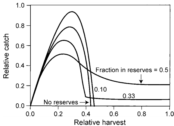
FIG. 1. Results from a model with 24 subpopulations linked by larval dispersal (Quinn et al. 1993) illustrate Principle 2 regarding the similarity of the effect on yield of increasing reserves to that of reducing harvest rate. At low harvest rates (fraction removed from fished area per year), relative catch (number removed plotted on an arbitrary scale) is reduced by increasing the fraction of subpopulations in reserves to a third or half (every third or every other population, respectively), but this is the fraction necessary to sustain the population at high harvest rates (redrawn from Quinn et al. [1993]).
