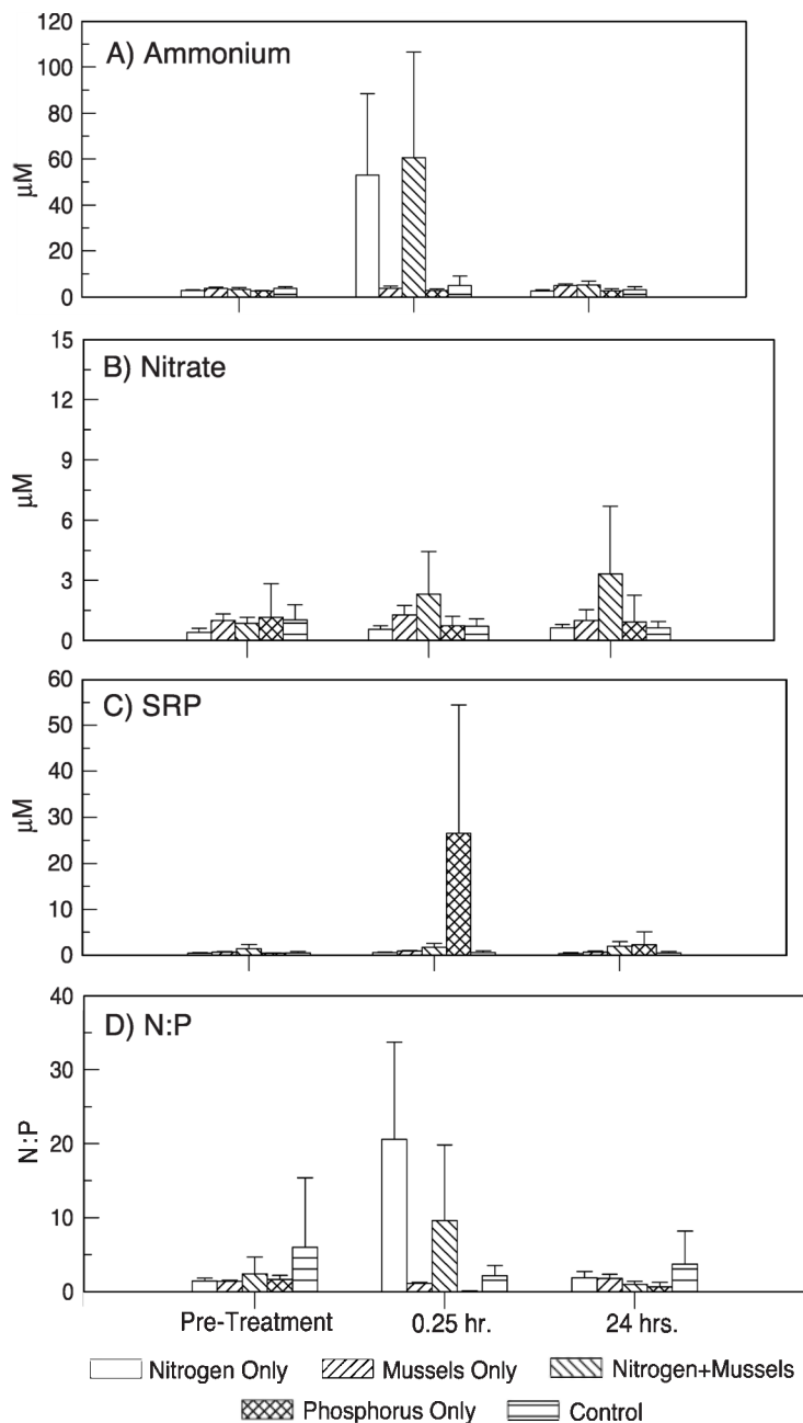
Fig. 8. Dissolved nutrient concentrations for all experimental tidepools throughout the experiment. Error bars represent the 95% confidence intervals.
