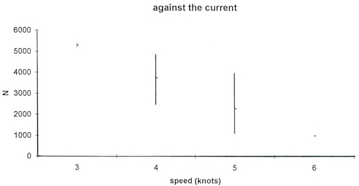
Fig. 3.3.5. Pressure force limits.
