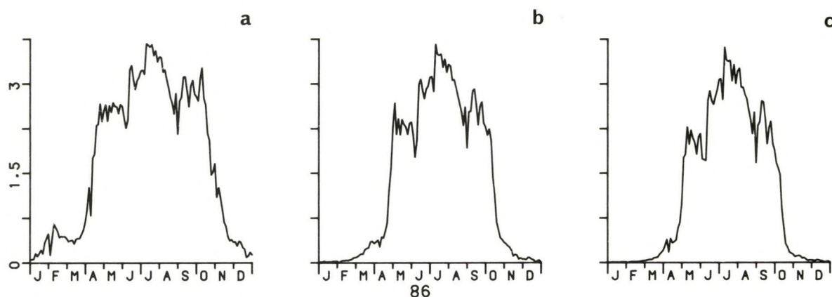
Fig. 7. Total pelagic primary production ( 10^6 \text{ kg C} ) simulated with a P and Si load from Lake IJssel equal to a: 0; b: the standard situation; c: 1.5 times as large as in the standard situation.
