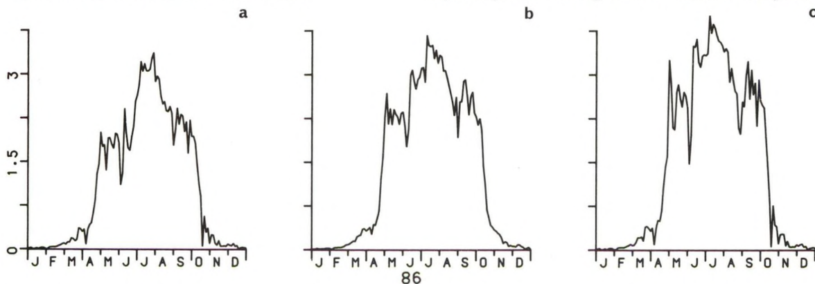
Fig. 5. Total pelagic primary production (10 6 kg C) according to the model simulations. a: reduced sediment load; b: standard situation; c: increased sediment load.
