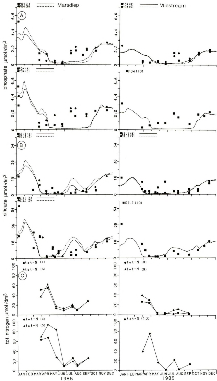
Fig. 3. Model simulation (lines) and measured concentrations (symbols) of (A) inorganic phosphate, (B) silicate and (C) nitrogen (NO 3 + NO 2 , only measured data) of a series of selected compartments representing the inner and outer compartments of the Marsdiep and Vliestream basins. Compartment numbers are indicated in brackets (see Fig. 1).
