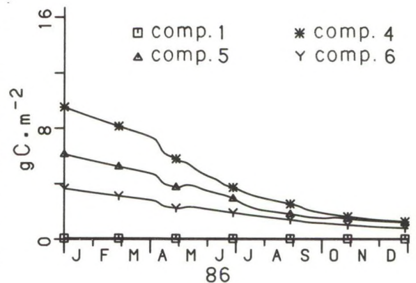
Fig. 9. Biomass of benthic suspension feeders in the subtidal ( \text{gC} \cdot \text{m}^{-2} ) in compartments 1, 4, 5 and 6 with increased initial values on Jan. 1.
