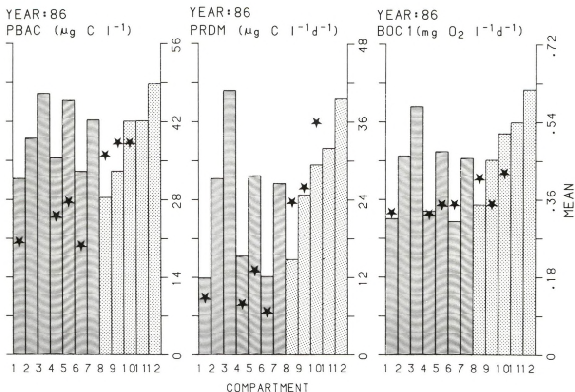
Fig. 12. Simulated mean annual bacterial biomass in \mu\text{g C}\cdot\text{dm}^{-3} (left), production in \mu\text{g C}\cdot\text{dm}^{-3}\cdot\text{d}^{-1} (middle) and BOC 1 in \text{mg O}_2\cdot\text{dm}^{-3}\cdot\text{d}^{-1} (right) in the compartments 1 to 12, respectively in 1986. Mean annual values of field data are also given (symbols).
