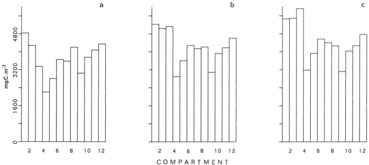
Fig. 8. Mean biomass of benthic suspension feeders in the intertidal ( \text{mgC} \cdot \text{m}^{-2} ) in the various compartments in April-September simulated with a P and Si load from Lake IJssel equal to a: 0 b: the standard situation; c: 1.5 times as large as in the standard situation.
