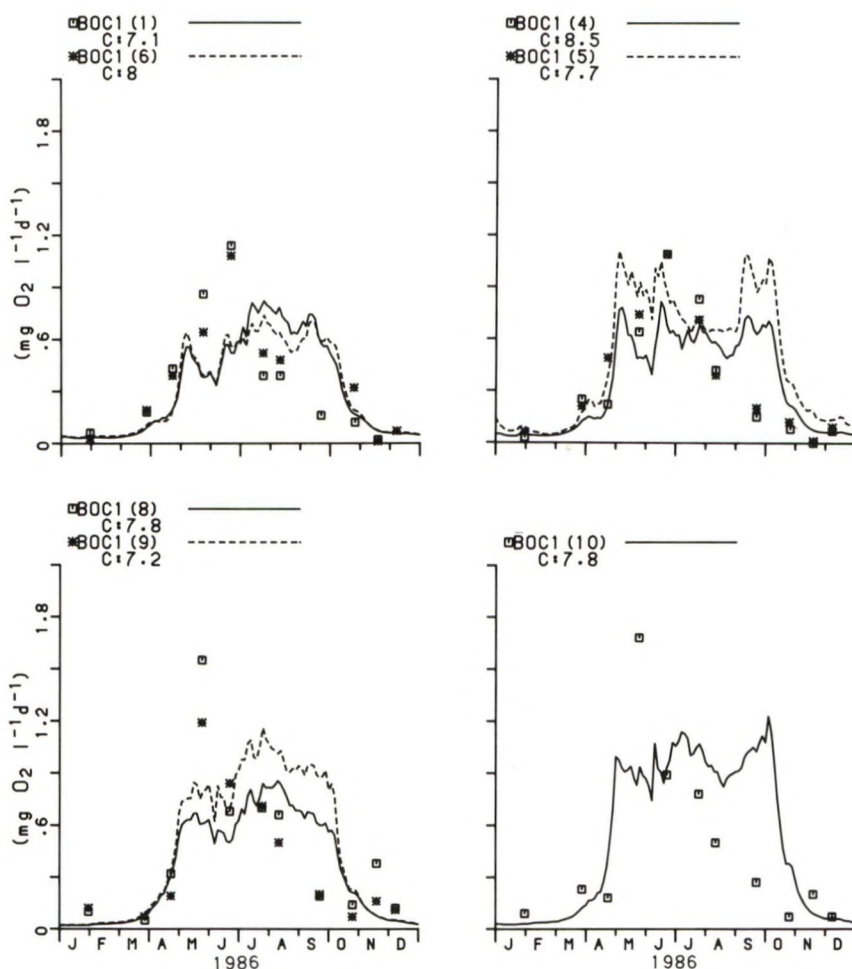
Fig. 11. Model simulations of the oxygen consumption ( \text{BOC}_1 ) of the water column in each of the 7 compartments 1, 4, 5, 6, 8, 9, 10 (lines) and field data (symbols) in \text{mg O}_2 \cdot \text{dm}^{-3} \cdot \text{d}^{-1} in 1986.
