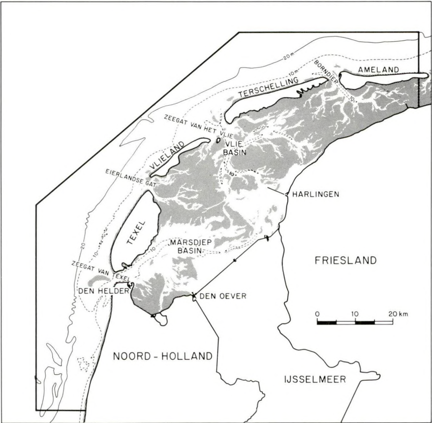
Fig. 1. (a) Location of the boundaries of the models with 3200 m and 500 m grid size. Results of the 500 m model are discussed in this article. (b) Map showing the boundaries and some isobaths (10 m, 20 m) of the 500 m model. Shaded areas represent tidal flats.
