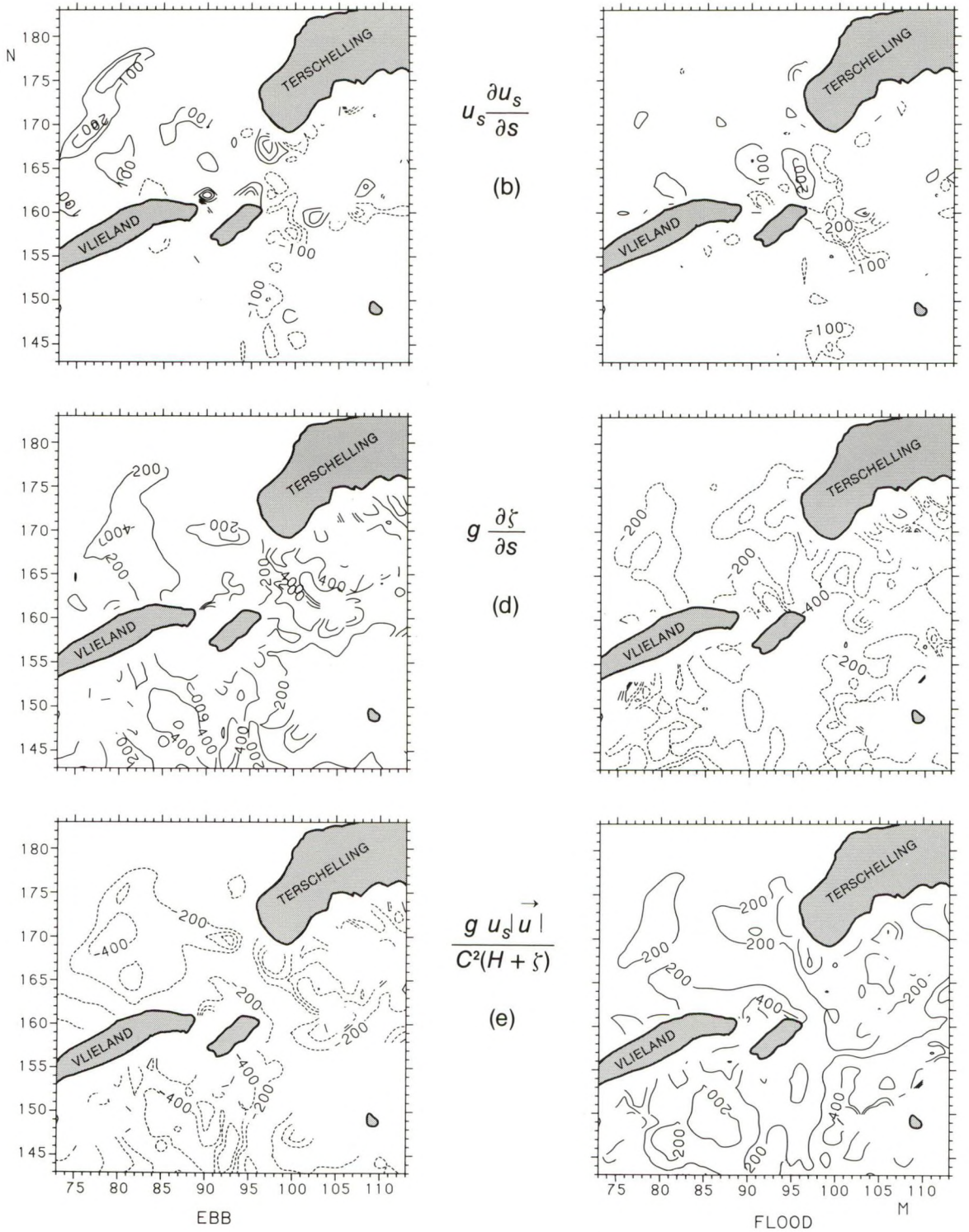
Fig. 9. (a) Isolines of the magnitude of terms b, d and e ( 10^{-6}\text{ms}^{-2} ) in equation (9), parallel to the local momentary streamline. On the left-hand side at the time of maximum ebb, in which the positive s-axis has the same orientation as during the flood, and on the right-hand side at the time of maximum flood. Solid lines represent isolines with positive values; dashed lines represent the same range of negative values (see text).
