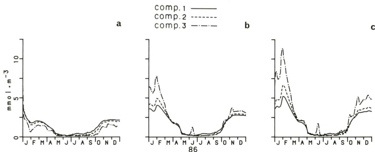
Fig. 6. Concentrations of dissolved reactive phosphate ( \text{mmol} \cdot \text{m}^{-3} ) in the compartments 1, 2, 3 according to the model simulations. a: no discharge from Lake IJssel; b: standard situation; c: discharges 1.5 times as large as in the standard situation.
