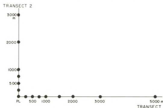
Fig. 2. Positions of the sampled stations on the transects (PL=platform). Distance in meters.
