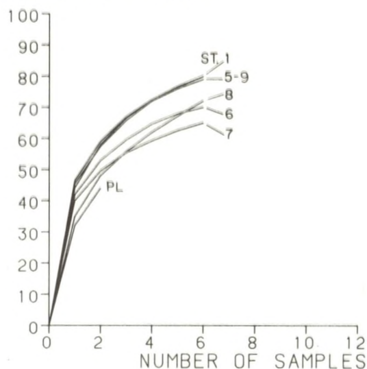
Fig. 5. Rarefaction curves of all stations from platform L4a, survey September.
