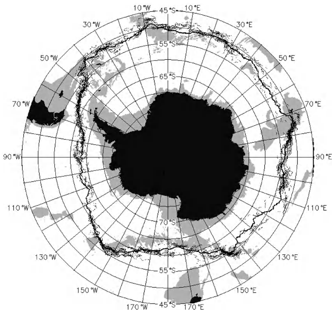
Fig. 1. Displayed are the long-term, mean position of the Antarctic Polar Front (thick black line) and the weekly positions used in this study from the October–March period for the 1997–1998 and 1998–1999 seasons. Gray shaded areas indicate ocean depth < 3000 m (bathymetry from Smith and Sandwell, 1994).
