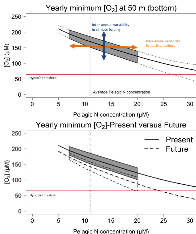
Fig. 11. Effect of increasing pelagic nitrogen concentration on the yearly minimum oxygen concentration ( [O_2] ) at 50 m depth (bottom). The current average pelagic nitrogen concentration ( 11 \mu\text{M} ) is indicated with a vertical dashed line. The horizontal red line at 63 \mu\text{M} indicates the hypoxia threshold. Top panel: using present climate forcings (year 2000). The dotted lines indicate the minimum and maximum concentration of the different climate simulations of 2000; polygon indicates the likely area of oxygen concentrations. The arrows indicate the interannual variability in climate forcings and nutrient loadings. Bottom panel: comparison between present (year 2000) and future climate forcings (year 2100). The polygon is grey for the present climate forcings and transparent (dotted line) for the future climate forcings.
