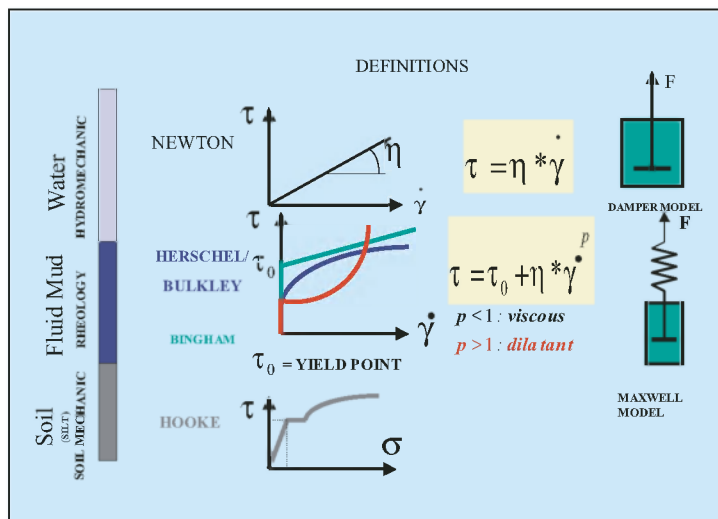
Figure 3. Definitions of fluid mud, comparing the laws of Newton, Herschel/Bulkley, Bingham and Hooke.
