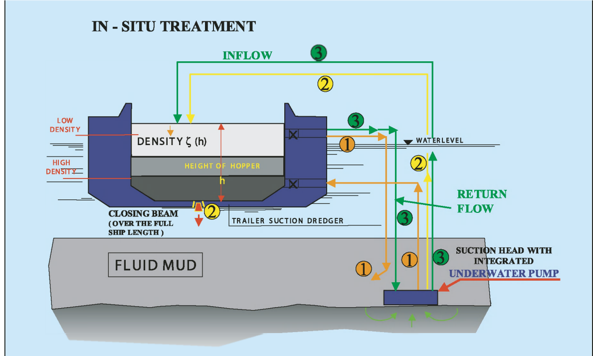
Figure 9. Three possibilities of in situ treatment.
