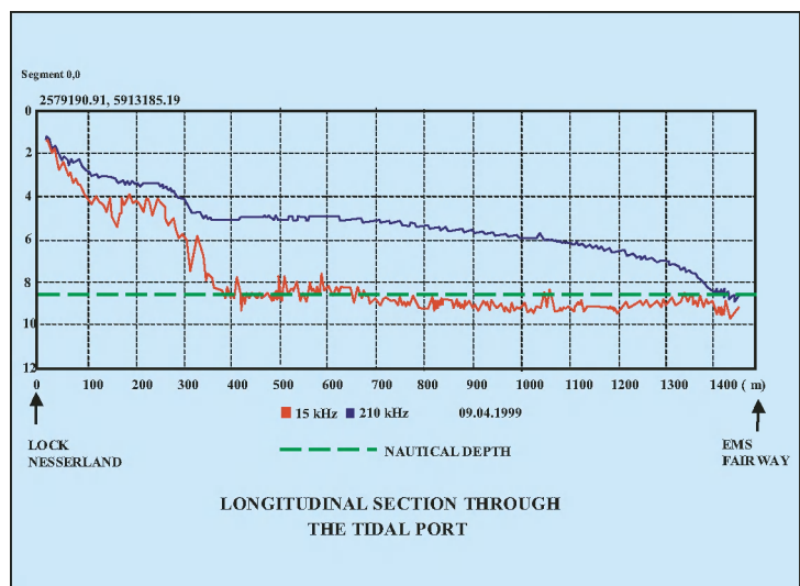
Figure 2. Longitudinal section through the Outer Harbour of Emden demonstrates the interrelations amongst adjoining harbours.
