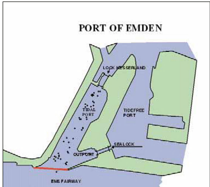
Figure 1. Location of area to be maintained at the Port of Emden.
