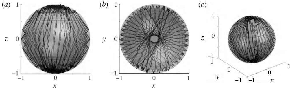
FIGURE 12. As in figure 4, example of a non-converging trajectory, corresponding to the star in figure 9(b). Here \eta = 0.9 , \omega = 0.5842 , x_0 = 0.139 , \phi_0 = -2.042 and 1000 reflections are depicted.
