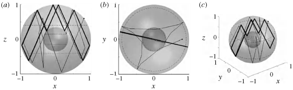
FIGURE 6. As figure 4, but for a meridional attractor in the three-dimensional shell ( \eta = 0.35 ). Here the ray at \omega = 0.4051 is launched at x_0 = 0.8 , \phi_0 = -7\pi/8 . The thick line marks the closed cycle of the final wave attractor. This trajectory also constitutes an example of a polar three-dimensional attractor (see the text).
