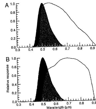
Fig. 2. Laboratory emission spectra of bioluminescent bacteria (black area) compared with spectral response functions. Data are shown for the U.S. Defense Meteorological Satellite Program OLS nighttime visible band of the sensor used in this study (A) and the proposed National Polar-orbiting Operational Environmental Satellite System Visible/Infrared Imager/Radiometer Suite day/night band (B). Regions of spectral overlap are shown in gray.
