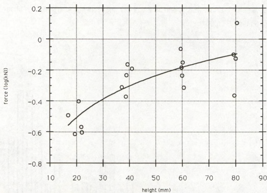
Figure 6: The relation between shell height and the force needed to crush it. Through the points a logarithmic regression is fitted; y = -1.4 + 0.7 \log(X) r = 0.8 ( p < 0.05 )
