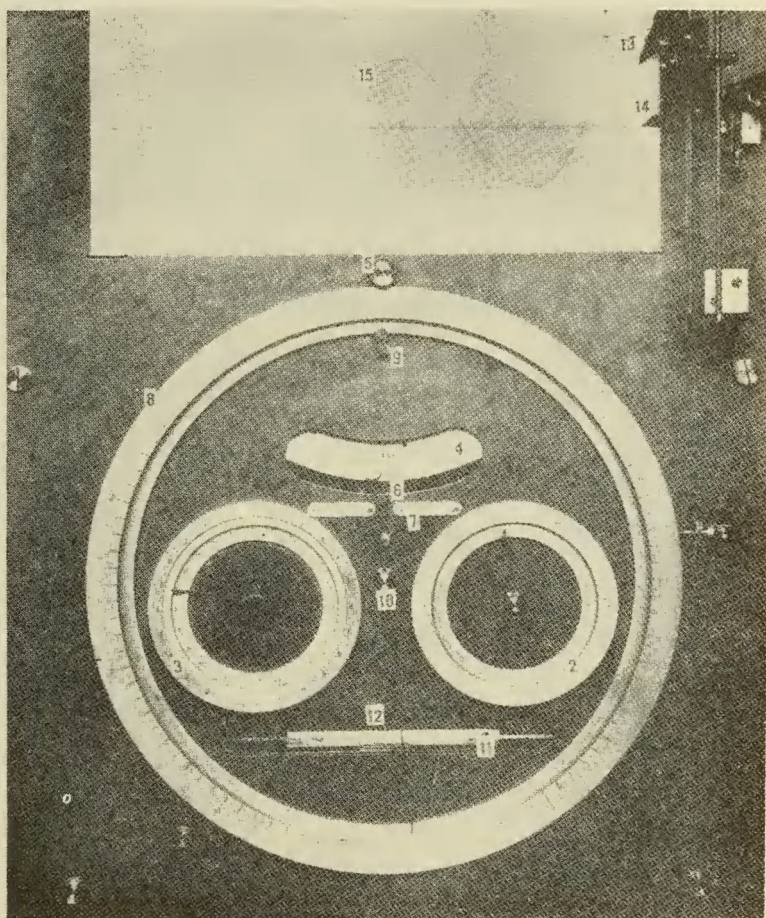
FIGURE 23.—TIDE-PREDICTING MACHINE, RECORDING DEVICES.
