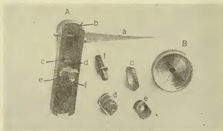
FIGURE 31.—TIDE-PREDICTING MACHINE, DETAILS OF CONSTITUENT CRANK.
