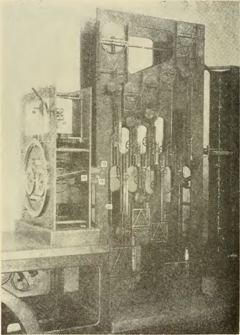
FIGURE 26.—TIDE-PREDICTING MACHINE, DIAL CASE FROM TIME SIDE.
