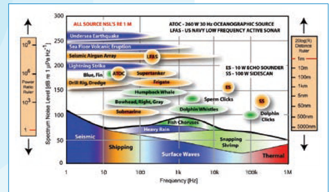
Fig. 1 The relationship of man made noise sources and naturally occurring sources of sound in the marine environment in terms of noise levels (dB re 1 \mu Pa Hz -1 ) and frequency (Hertz). © Seiche. Source 3
