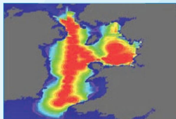
Figure 2b Output from an ambient noise model DTI SEA Area 6, October, with receiver at 10 m for a frequency of 1 kHz. Source 5
