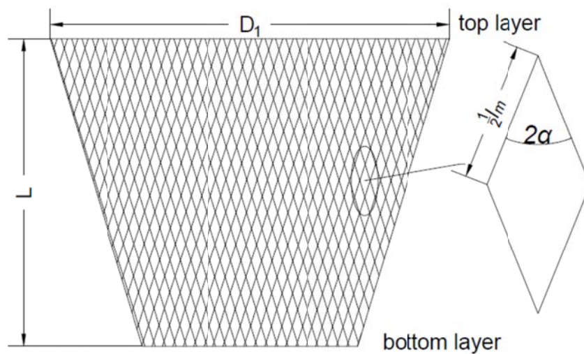
Figure 4.13 Definition of mesh properties.
