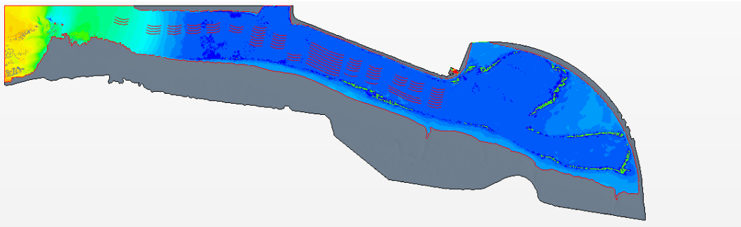
Figure 3.38 Impression of the free surface during the flood tide
