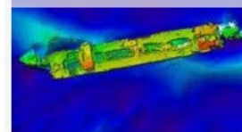
Multibeam sonar
