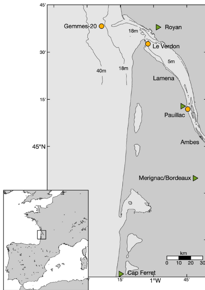
Fig. 1. Gironde Estuary, France. Green triangles represent the location of wind stations (Cap Ferret, Merignac/Bordeaux, Pauillac, and Royan). Dark yellow circles represent the location of turbidity data (from MAGEST program: Pauillac and Le Verdon, and from GEMMES buoy 20). Black contours represent the depth isobaths at 5m, 18m and 40m. (For interpretation of the references to colour in this figure legend, the reader is referred to the Web version of this article.)
