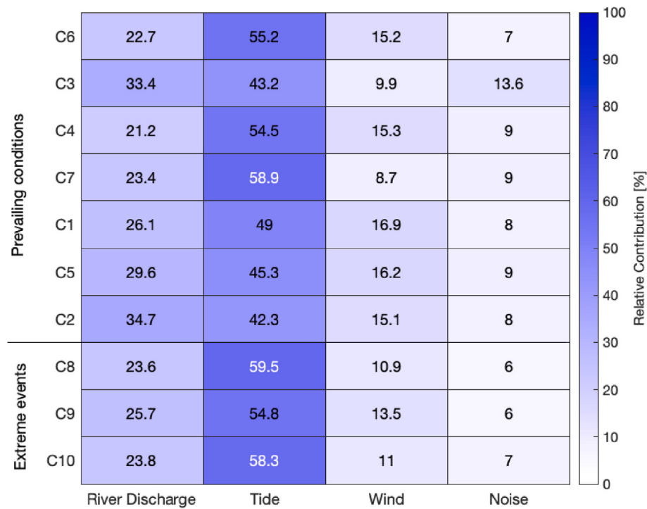
Fig. 4. Class-specific relative contribution (%) of predicting factors (river discharge, tide, wind and uncertainty or noise) for modeled surface SSC (database A). Classes C1–C7 depict relative contribution of forcing mechanisms under prevailing conditions (ordered from low (C6) to high (C2) log SSC), classes C8–C10 depict relative contribution of extreme events (extreme high river discharge, potential windbursts, and simultaneous extremes, respectively).
