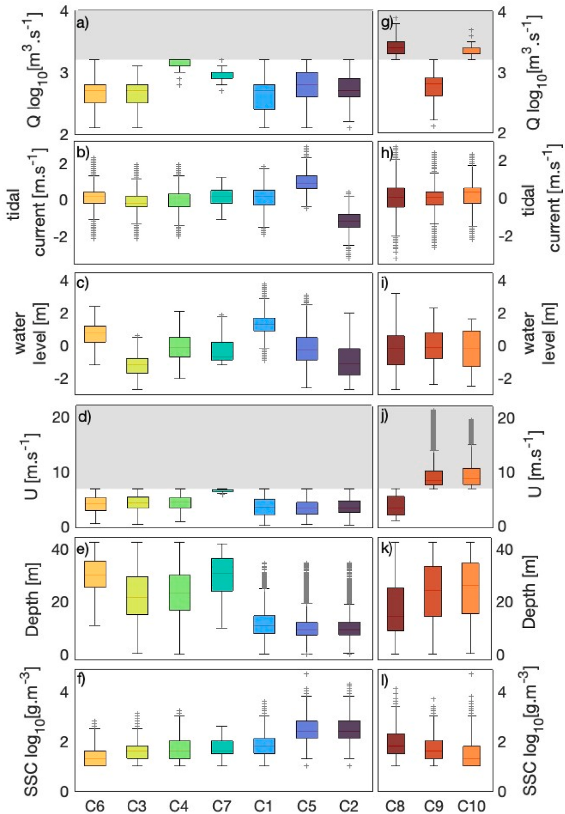
Fig. 3. Classes of coherent hydrodynamical and sedimentological patterns of database A (x-axis), for river discharge ( Q \log_{10} transformed; a,g), tidal current (b,h), water level (c,i), wind speed ( U ; d,j), depth (e,k) and model output of surface sediment concentration ( \text{SSC} \log_{10} transformed; f,l). Left panels (a–f) represent hydro-sedimentological classes under prevailing conditions, while right panels (g–i) represent classes under extreme event conditions (respectively simultaneous extreme river discharge, potential windburst, and simultaneous extreme river discharge and potential windburst). The shaded upper portion of (a,g) and (d,j) respectively represent the threshold defining occurrence of extreme river discharge ( Q_{\log_{10}} > 3.24 \text{ m}^3 \text{ s}^{-1} ) and potential windburst events ( U > 6.82 \text{ m s}^{-1} ) in the Gironde Estuary. Classes of prevailing conditions are ordered based on increasing SSC.
