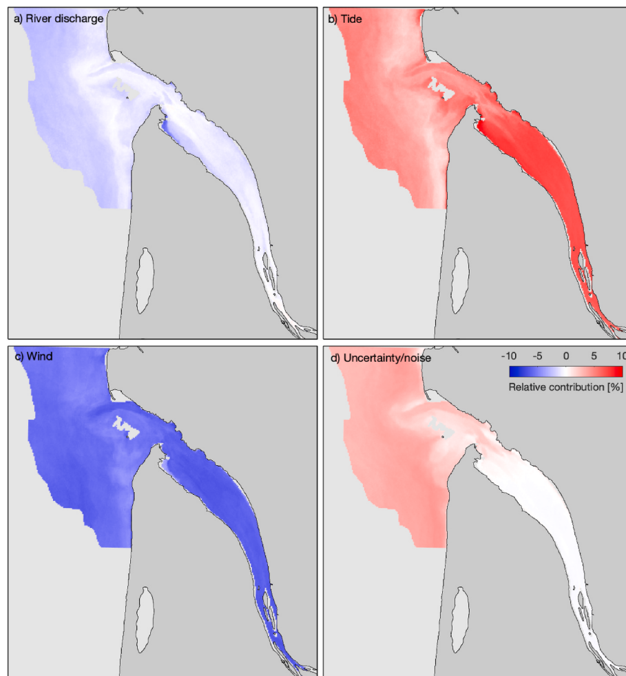
Fig. 6. Spatial difference between overall relative contribution for variability of surface sediment dynamics estimated from database A and database B. Red (blue) shades indicate higher overall relative contributions estimated from database A (B). (For interpretation of the references to colour in this figure legend, the reader is referred to the Web version of this article.)
