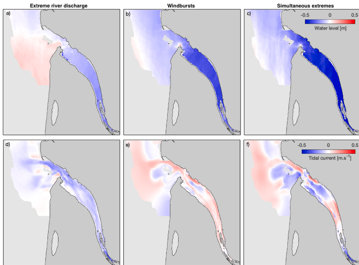
Fig. 7. Spatial difference between prevailing and extreme conditions of water level (a–c) and tidal current (d–f). Regions in blue (red) depict lowest (highest) water level or tidal currents under prevailing conditions. (For interpretation of the references to colour in this figure legend, the reader is referred to the Web version of this article.)
