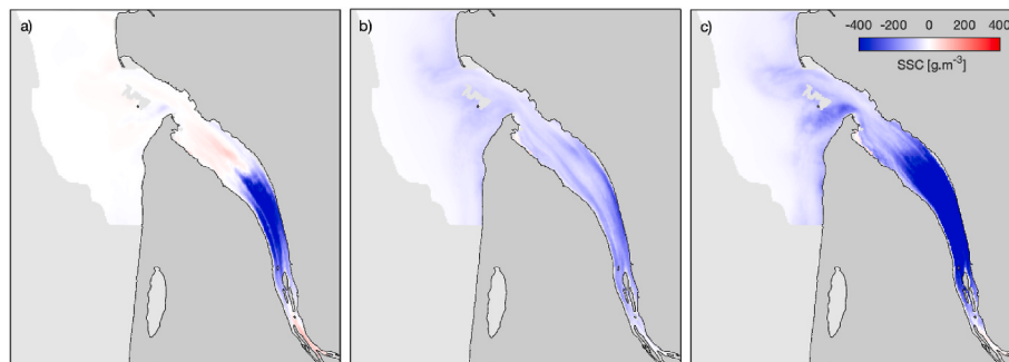
Fig. 8. Spatial difference between SSC under prevailing conditions and SSC under (a) extreme river discharge, (b) windbursts, and (c) simultaneous occurrence of extreme river discharge and windbursts. Regions in blue (red) depict lowest (highest) SSC under prevailing conditions. (For interpretation of the references to colour in this figure legend, the reader is referred to the Web version of this article.)
