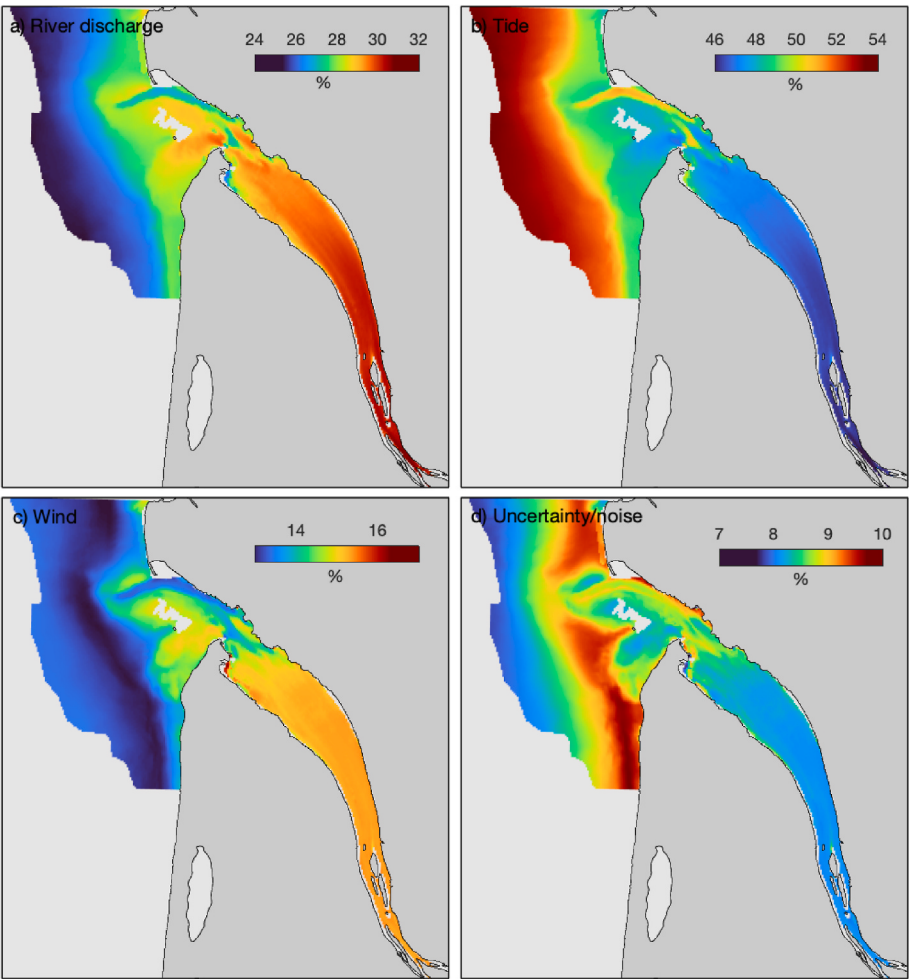
Fig. 5. Synoptical mean contribution of predicting factors for modeled surface SSC (database A): (a) river discharge, (b) tides, (c) winds and (d) uncertainties/noise to variability in surface suspended sediment concentrations. Attention to the different ranges of percentage on each subplot.
