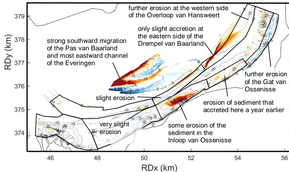
Figure 3.8 Bathymetric change of the Inloop van Ossensisse (July 2017 to January 2018)
