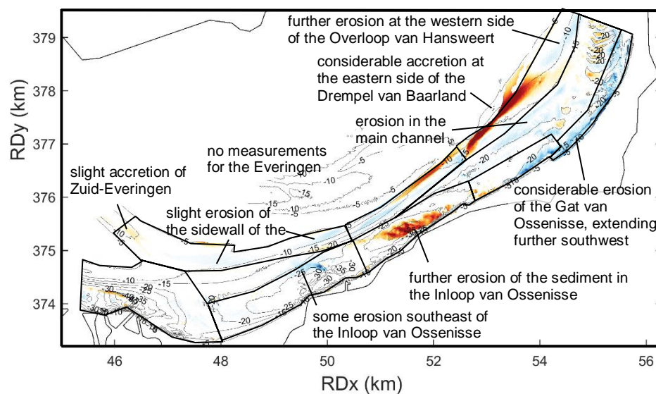
Figure 3.9 Bathymetric change of the Inloop van Ossensisse (January 2018 to February 2019)
