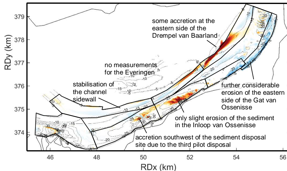
Figure 3.10 Bathymetric change of the Inloop van Ossensisse (February to June 2019)
