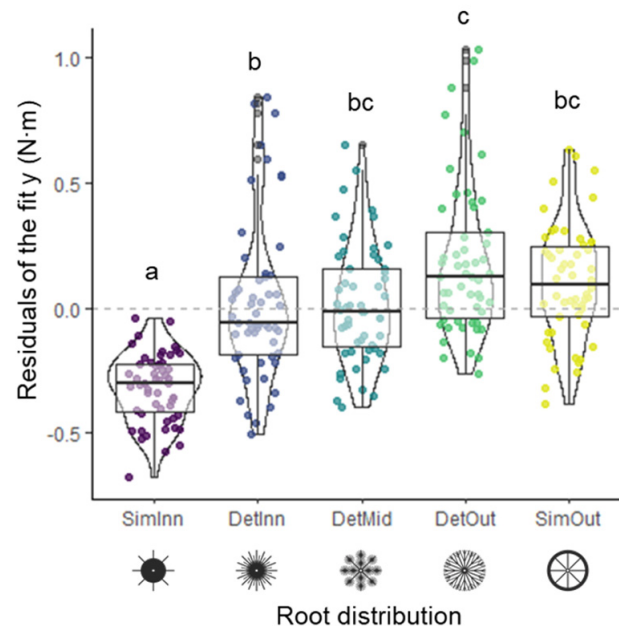
Figure A4. Residuals (jitterplot with boxplot and violinplot) of the linear regressions from Figure 7, showing the residuals of different root plates in different colours. Significance letters (a, b, bc, c) ( \alpha = 0.05 ) from Dunn's test. Breakages were half (25% of the complete plate) or complete (45%) breakage at the windward, leeward, or both sides of the root plate (see Figure 2b).
