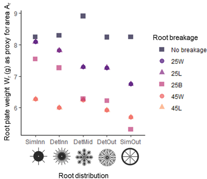
Figure 3. Root plate weight W_r (g), as a proxy for area A_r (cm 2 ), per root mass distribution and root breakage.
