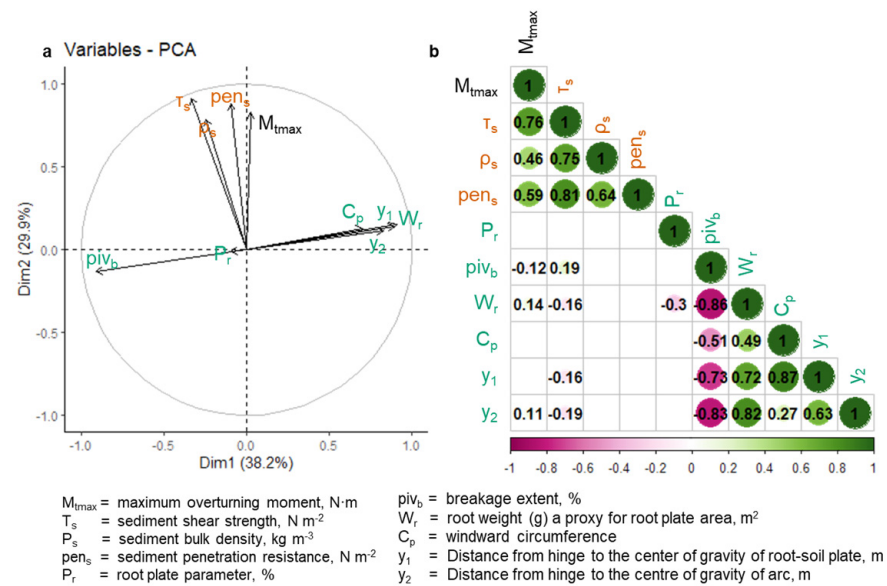
Figure A3. (a) Correlation circle showing correlation between variables and Principal Components and (b) all significant ( \alpha = 0.05 ) correlations between variables where darker greens represent a larger positive correlation, and darker pinks represent a negative correlation. Symbol colors indicate sediment (brown) and mimic (green)-related properties.
