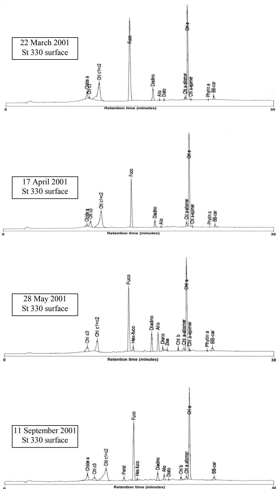
Figure I-7: Absorbance chromatograms (detection at 436 nm) of samples taken at four representative periods at station 330 of the Belgian coastal zone in 2001. Abbreviations refer to the pigment name in Table I-6.
