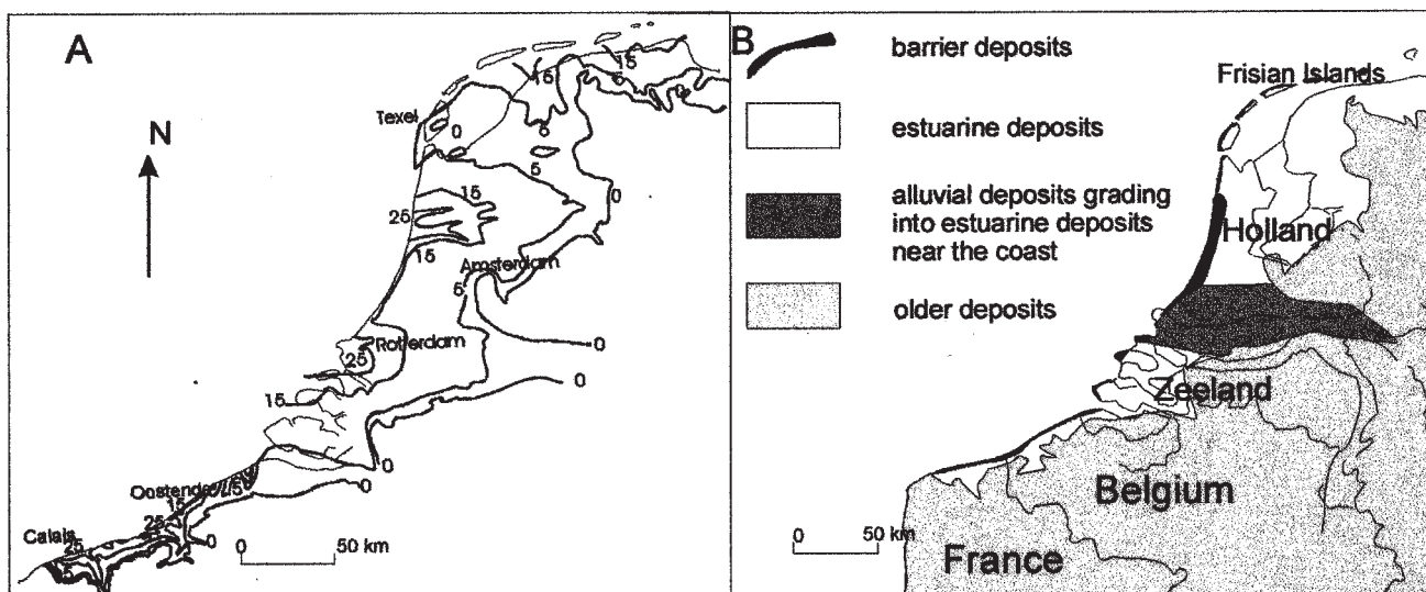
Fig. 2. Geological context.
