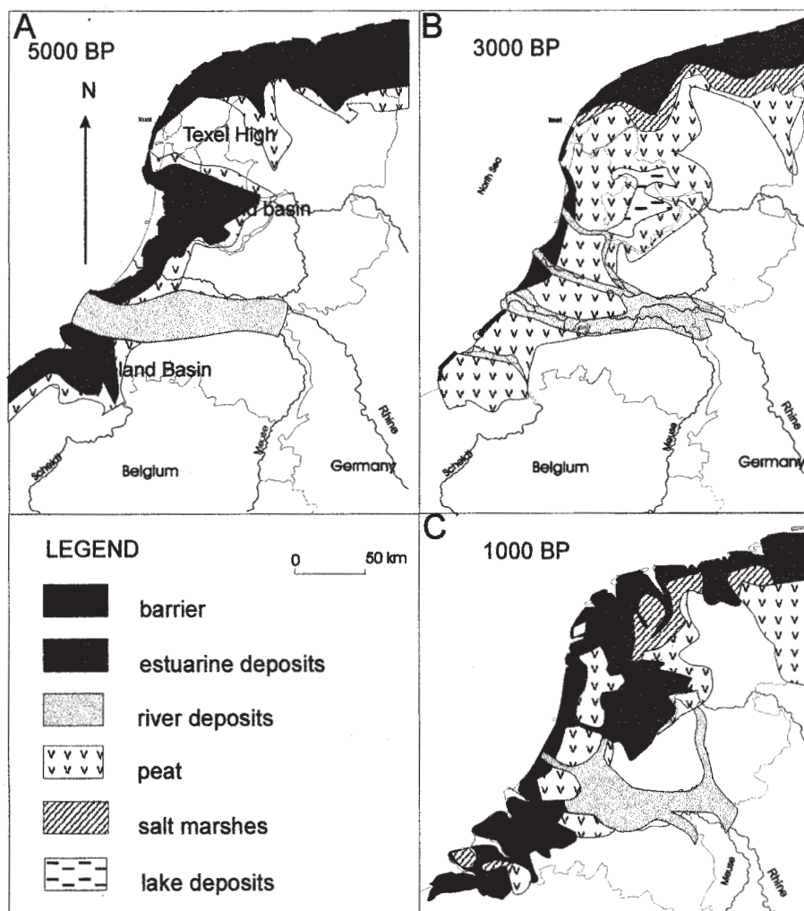
Fig. 5. Simplified paleogeography of the coastal plain of the Netherlands at approx. 5000 BP, approx. 3000 BP and approx. 1000 BP; modified from Zagwijn (1986).
